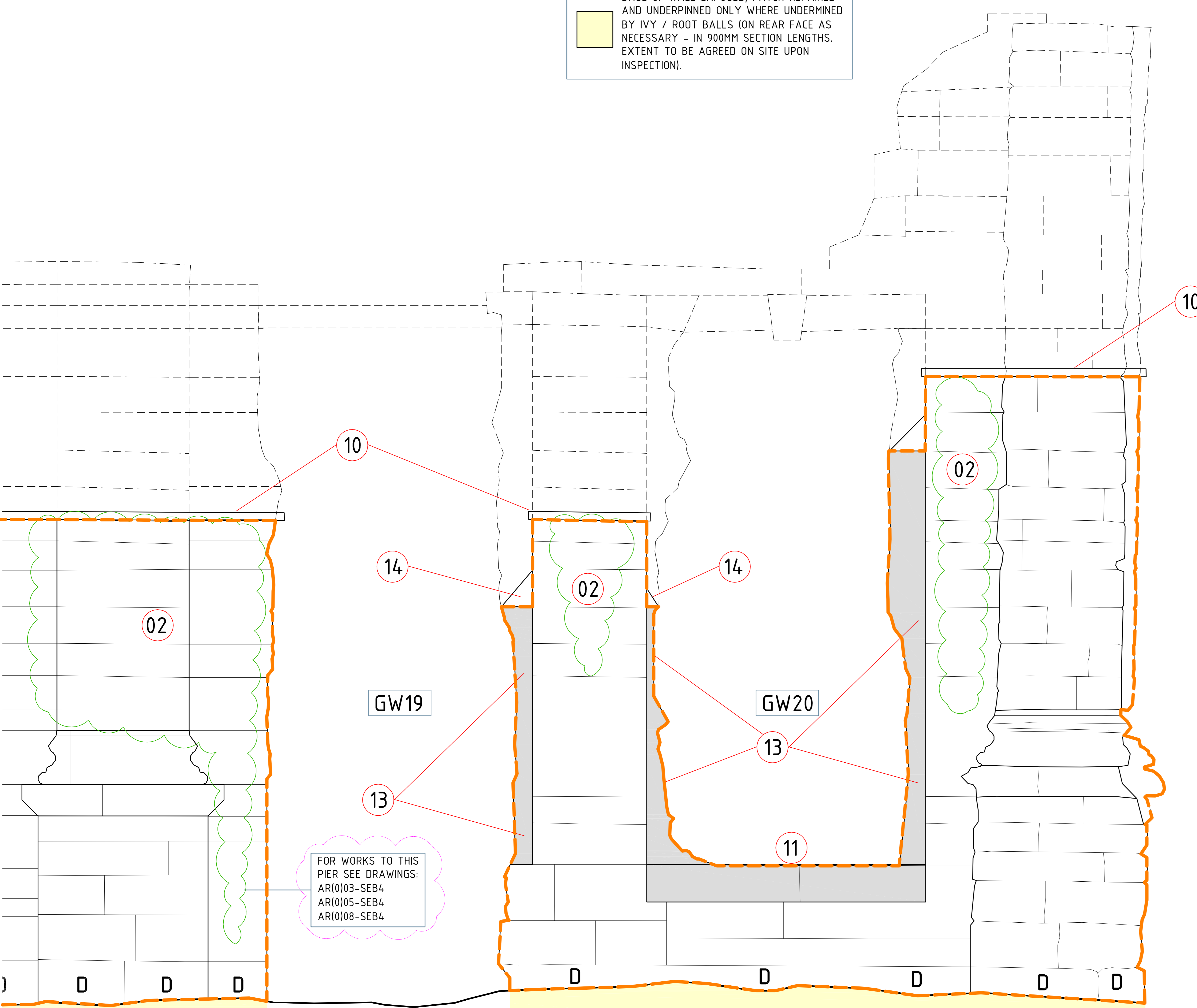
SEB5: PROPOSED EXTERNAL ELEVATION SCALE 1:10 @ A0
