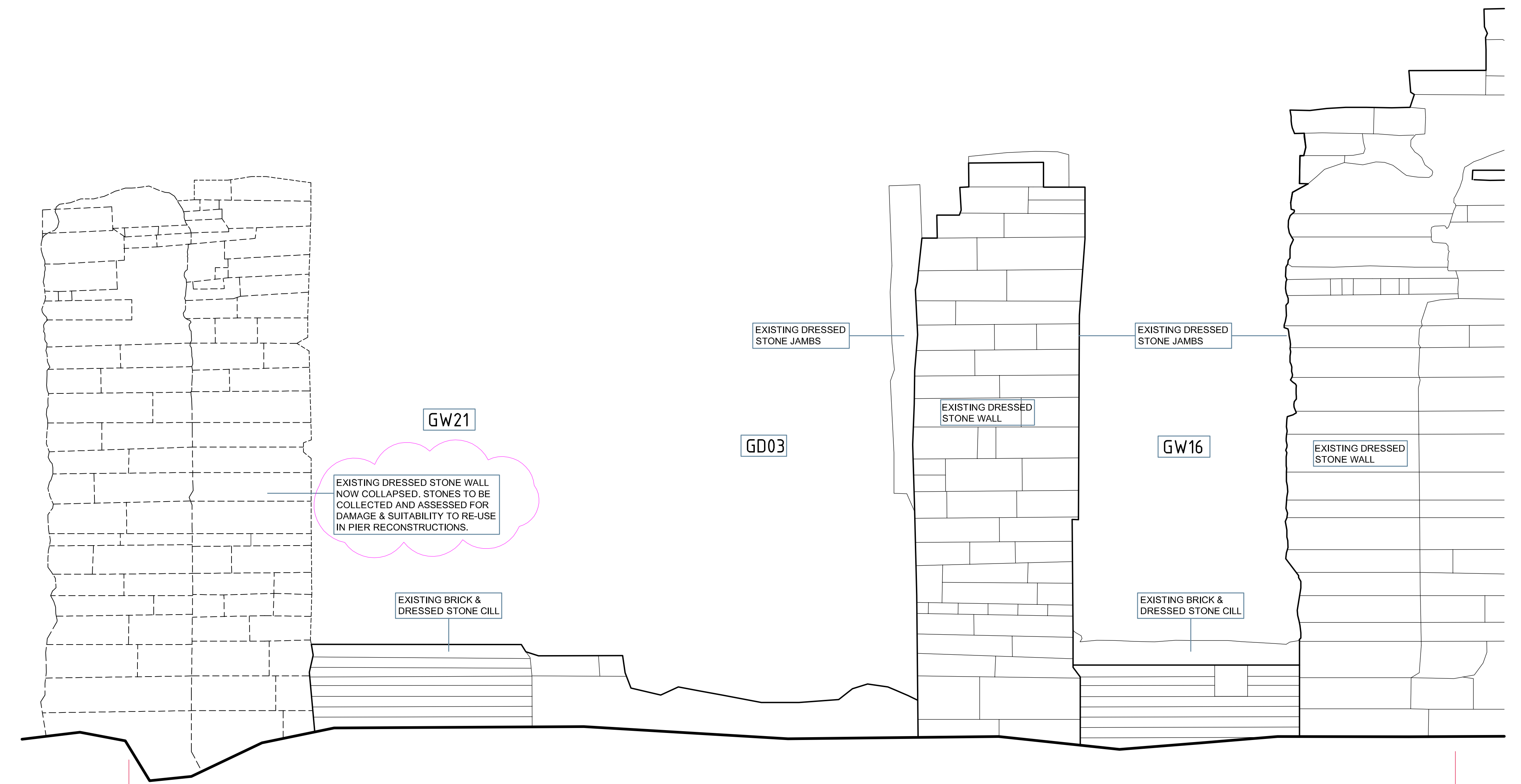
ELEVATION 5 - SEB3: EXISTING INTERNAL ELEVATION Scale 1:20 @ A0
