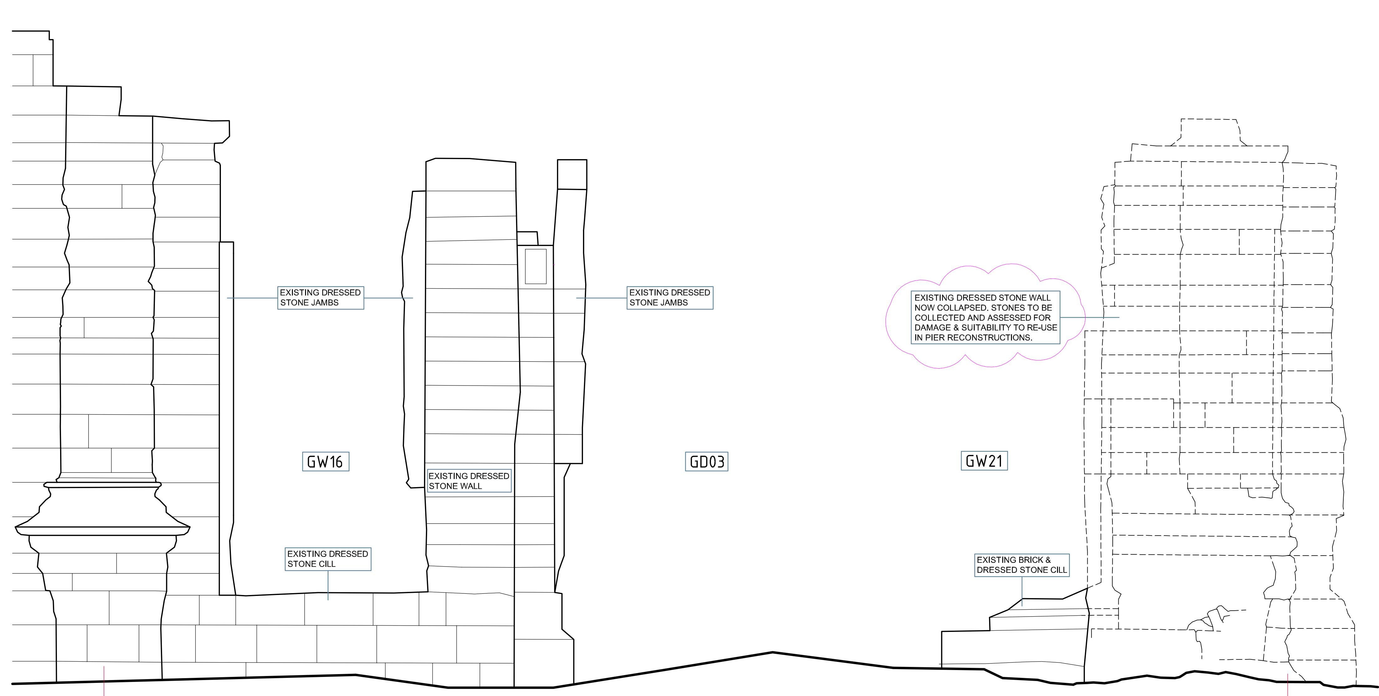
ELEVATION 3 - SEB3: EXISTING EXTERNAL ELEVATION Scale 1:20 @ A0
