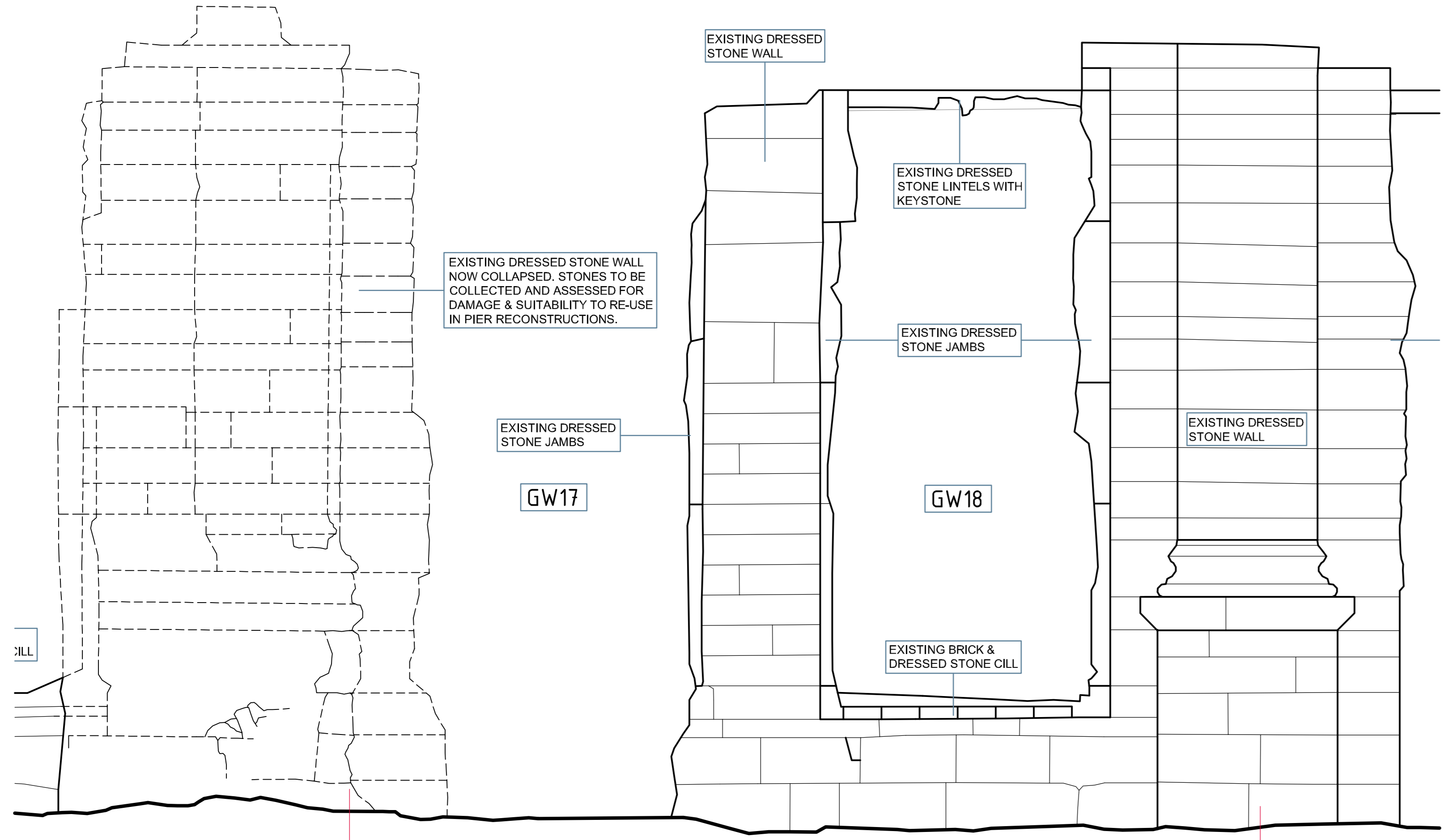
ELEVATION 3 - SEB4: EXISTING EXTERNAL ELEVATION Scale 1:20 @ A0
