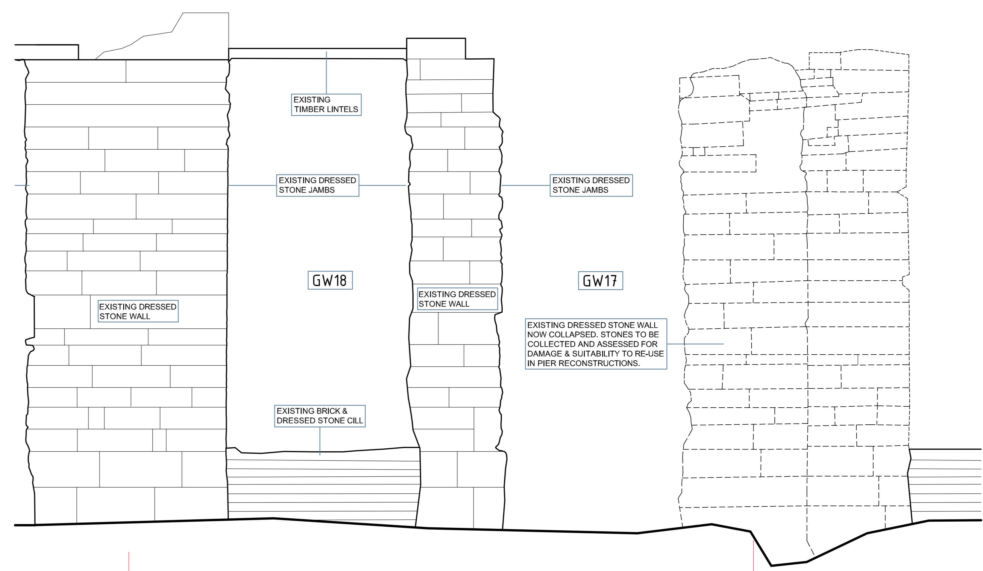
ELEVATION 5 - SEB4: EXISTING INTERNAL ELEVATION Scale 1:20 @ A0
