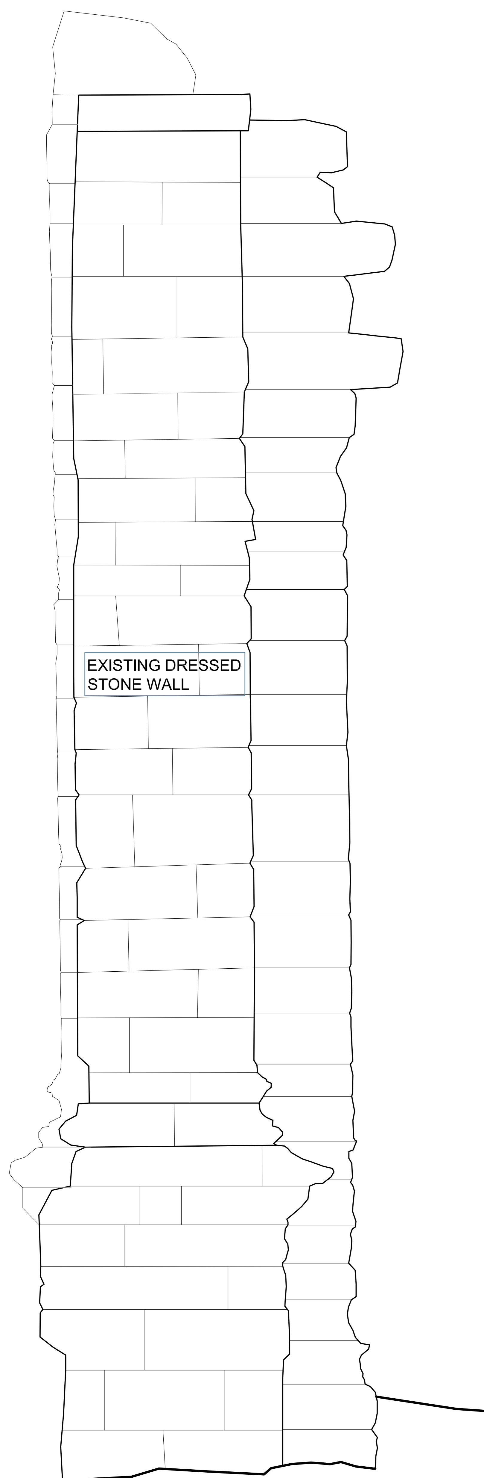
EXISTING SEB5 CORNER RETURN SCALE 1:20 @ A0
