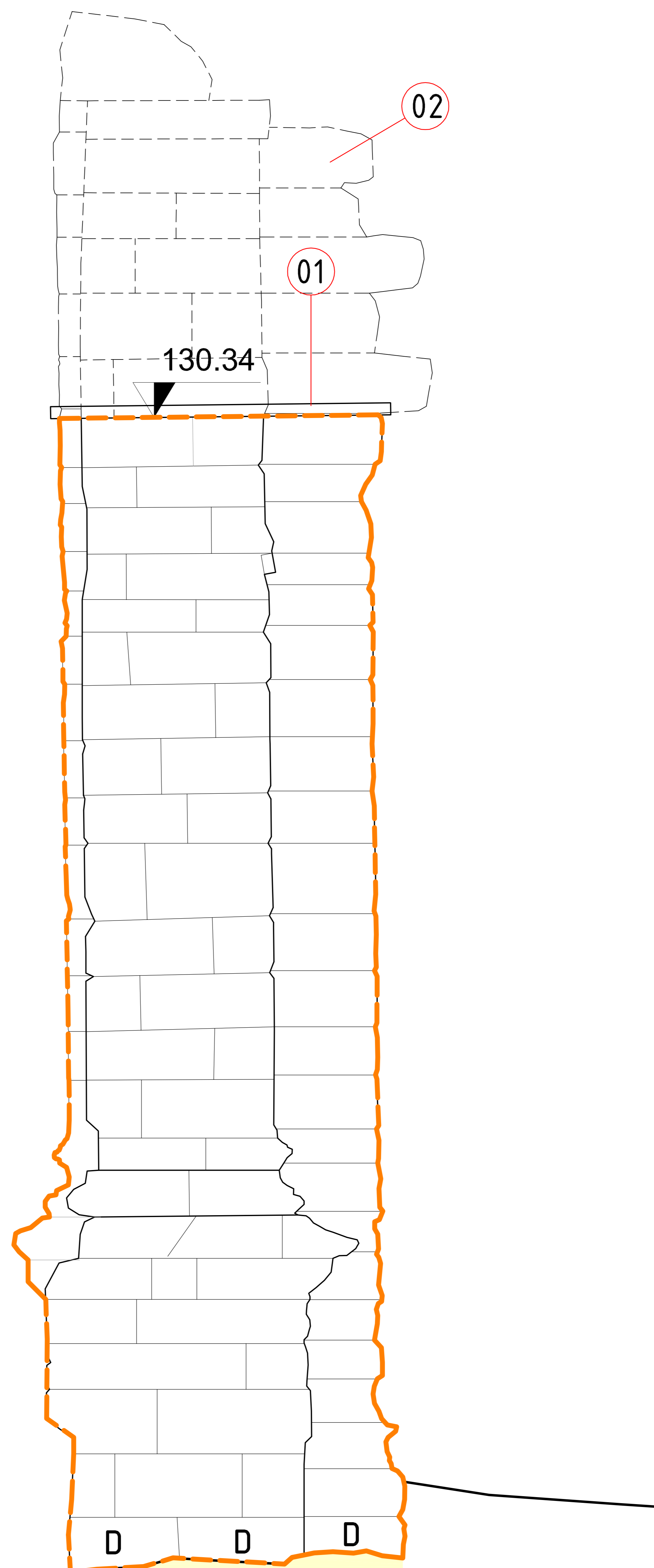
PROPOSED SEB5 CORNER RETURN SCALE 1:10 @ A0
