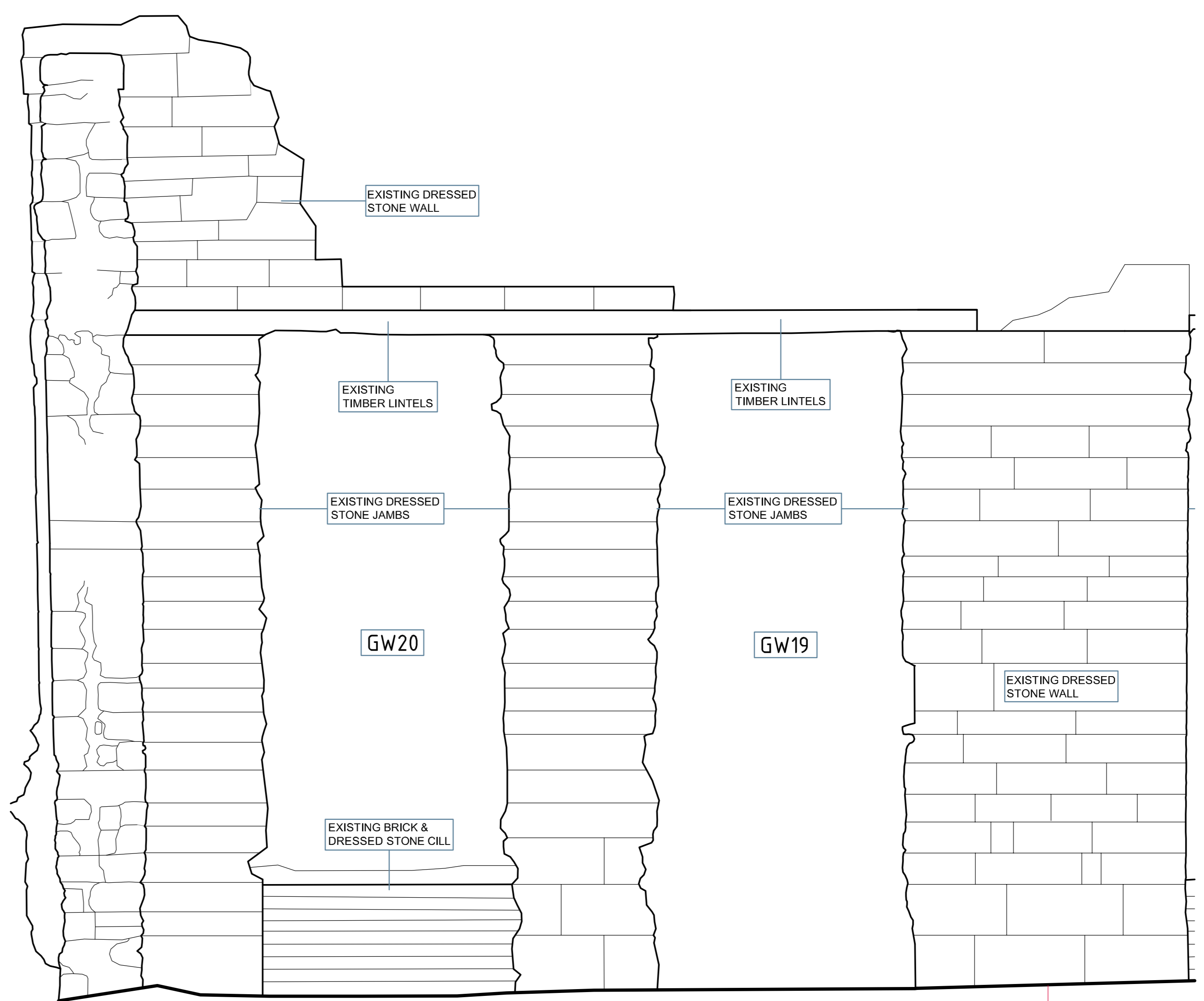
ELEVATION 5 - SEB5: EXISTING INTERNAL ELEVATION Scale 1:20 @ A0
