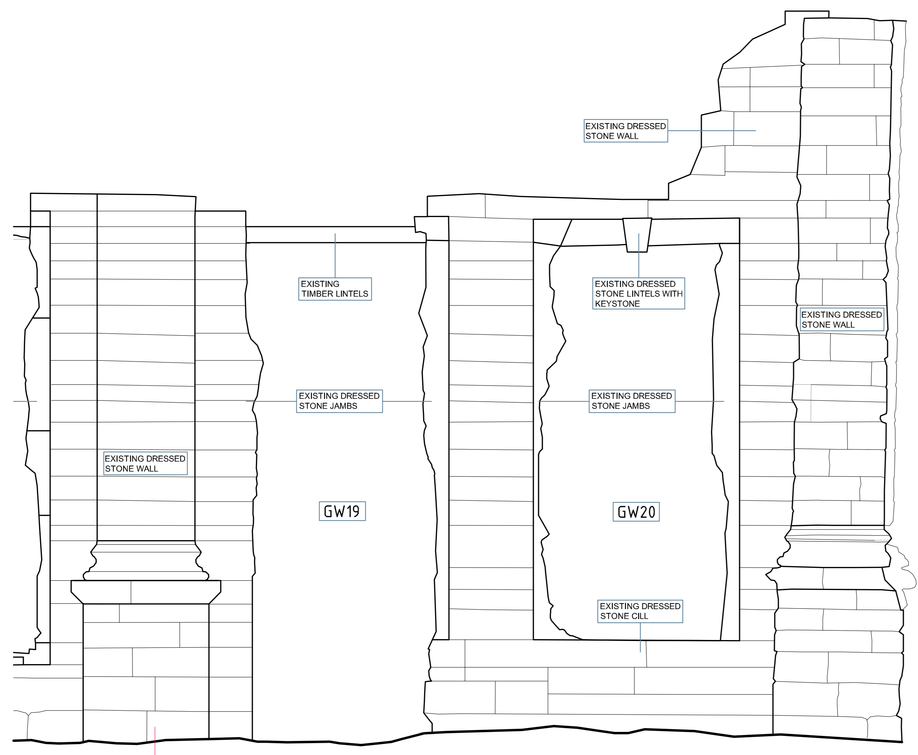
ELEVATION 3 - SEB5: EXISTING EXTERNAL ELEVATION Scale 1:20 @ A0
