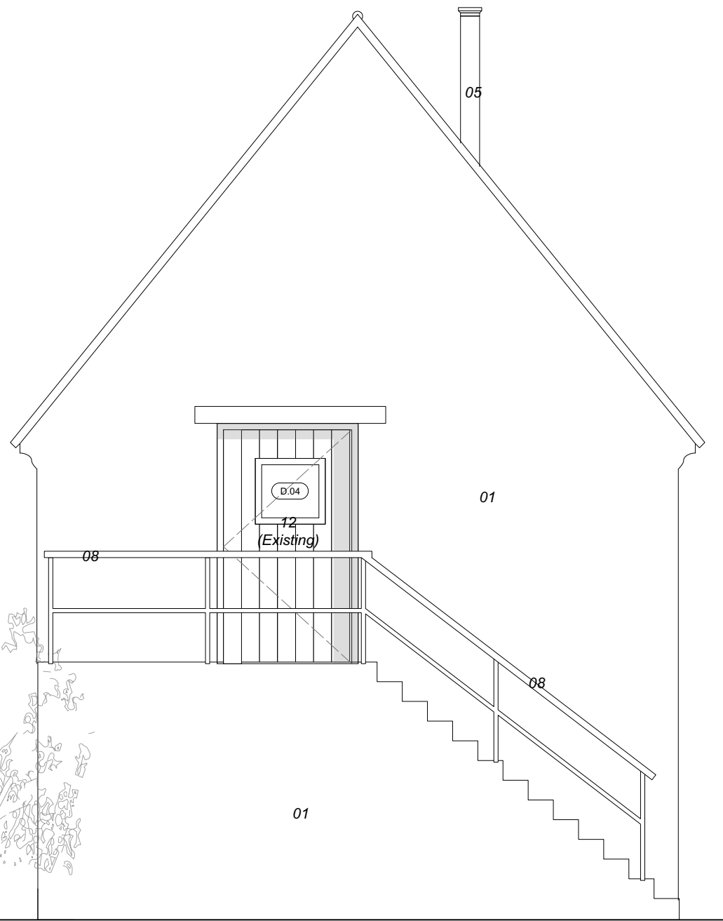
South Elevation
