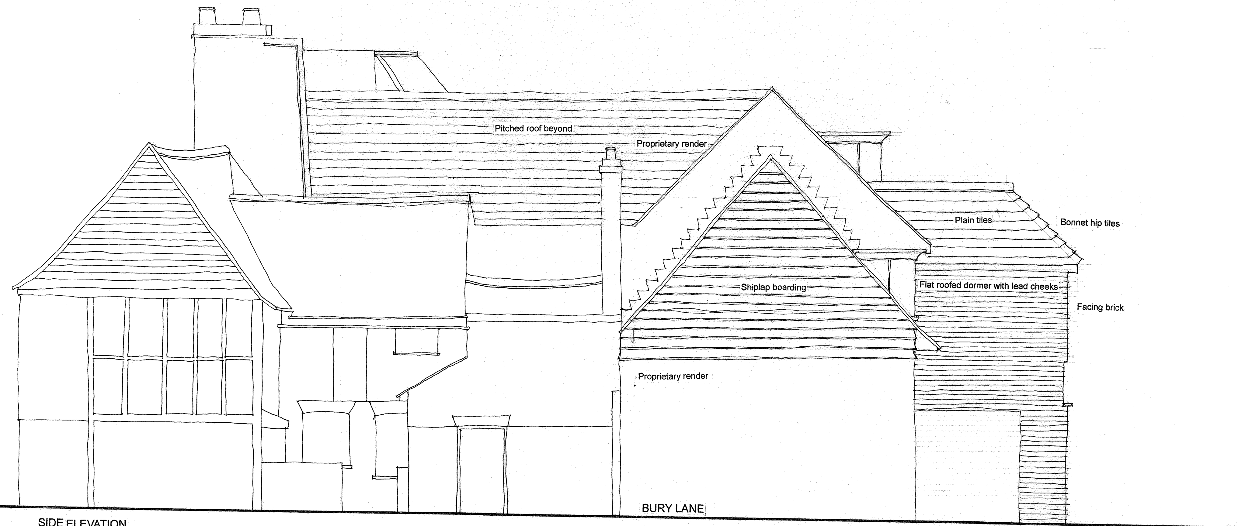
SIDE ELEVATION
