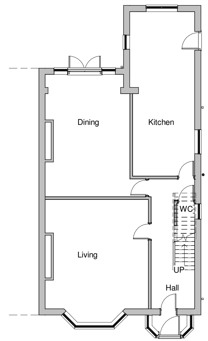
2 Ground Floor 1 : 100
