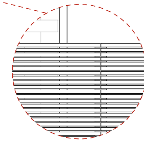
Slatted Fence Detail Scale: 1:25
