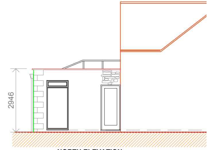
NORTH ELEVATION
