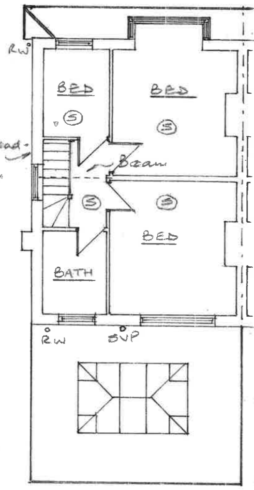
EXTG. 1ST. F. PLAN
