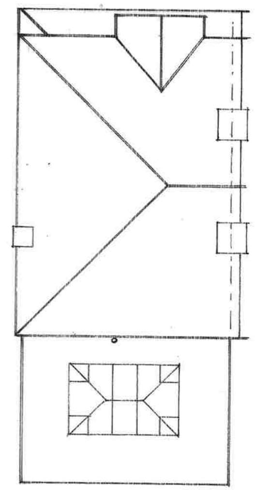
EXTG. ROOF PLAN
