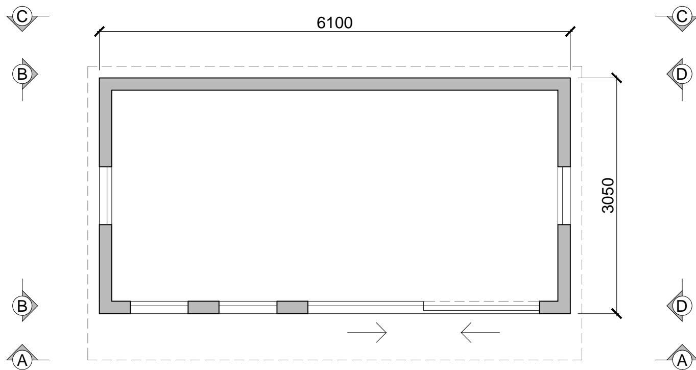
FLOOR PLAN
