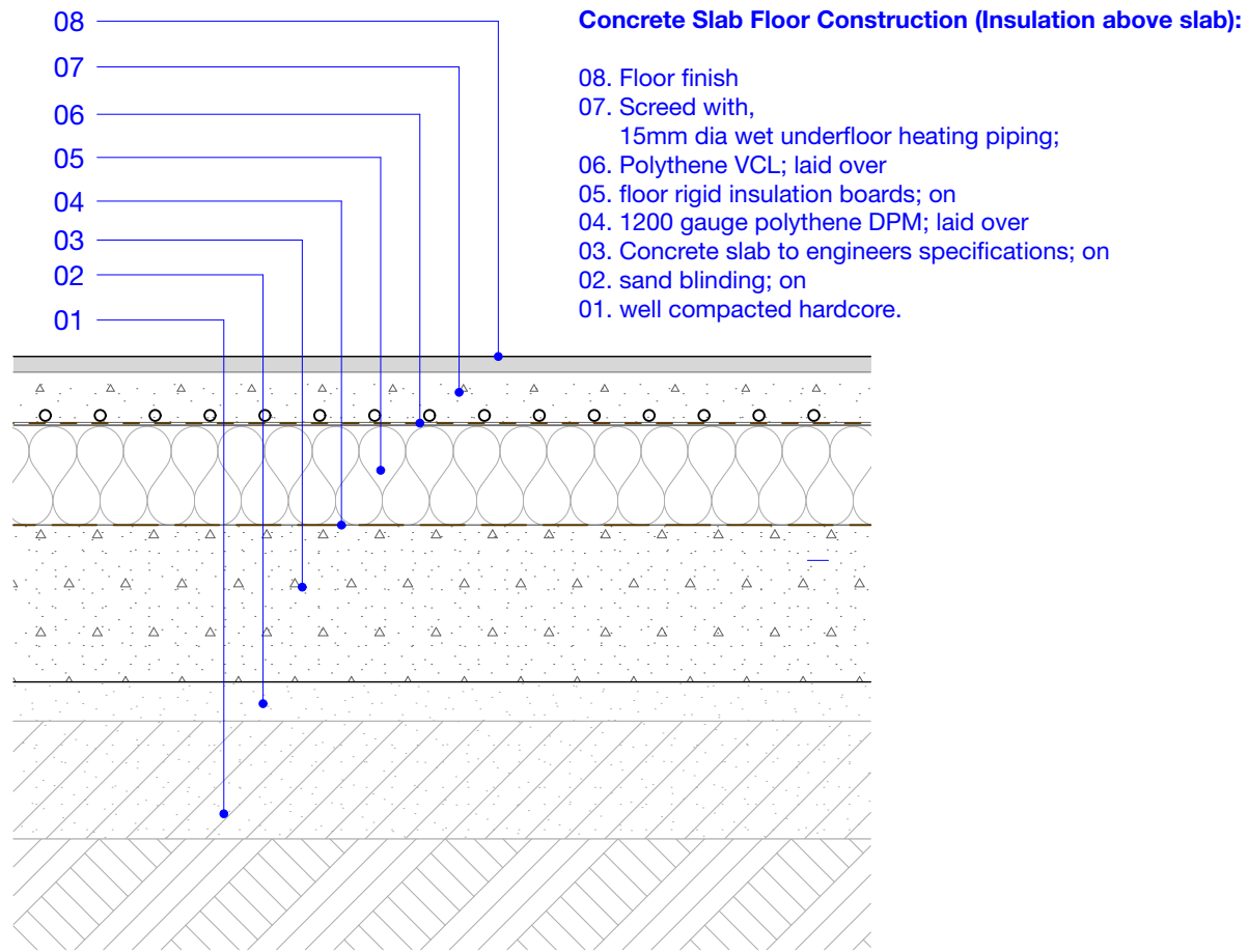
Typical Detail 01: Underfloor Heating to Lower Ground Floor 1:10
