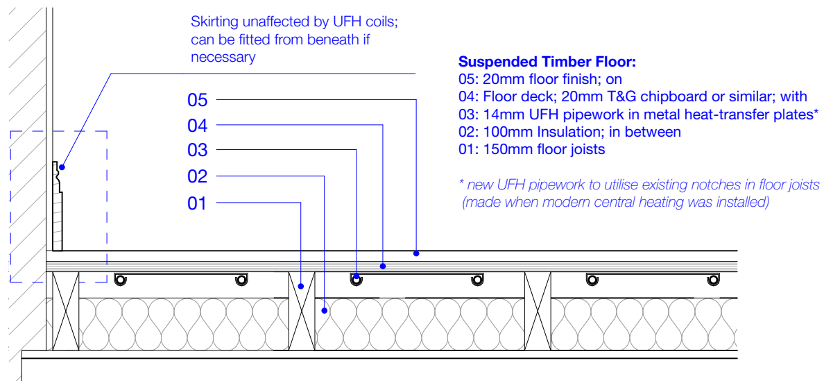
Typical Detail 02: Underfloor Heating to upper floors 1:10
