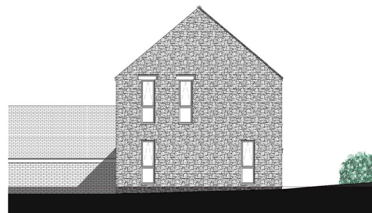
East Elevation. 1 : 100
