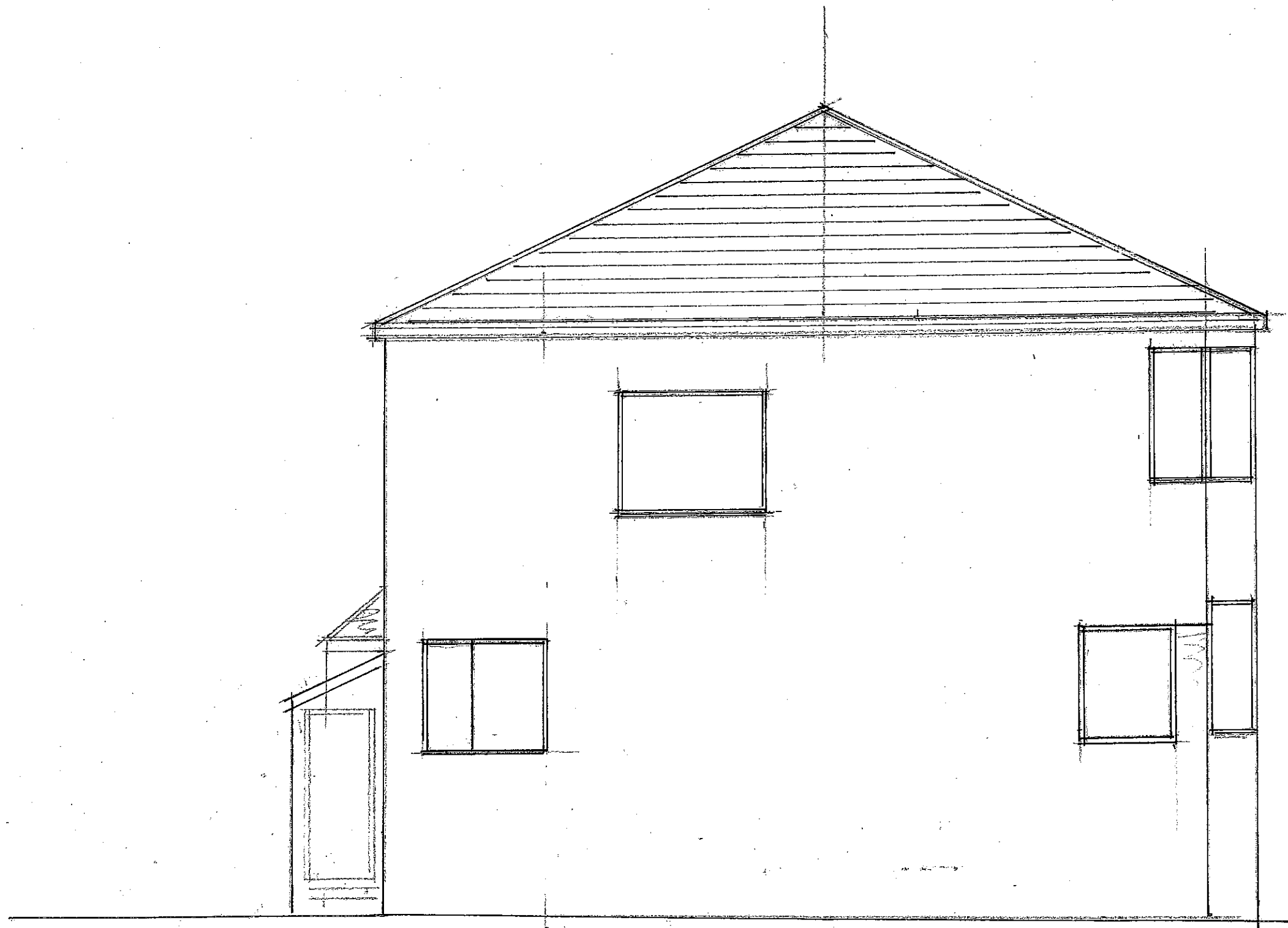
EXISTING SIDE ELEVATION 1:50 @ A3
