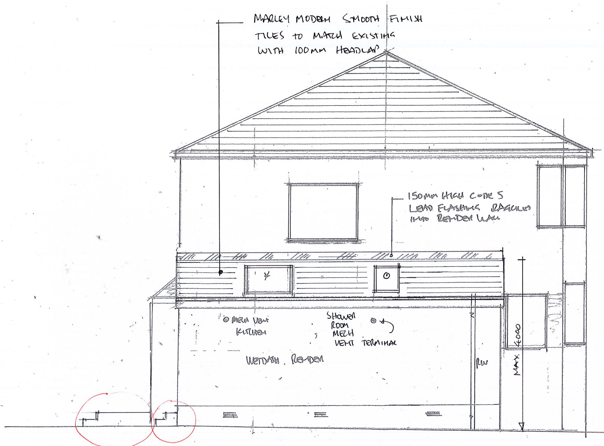
Proposed Side Elevation SCALE 1:50 @ A3
