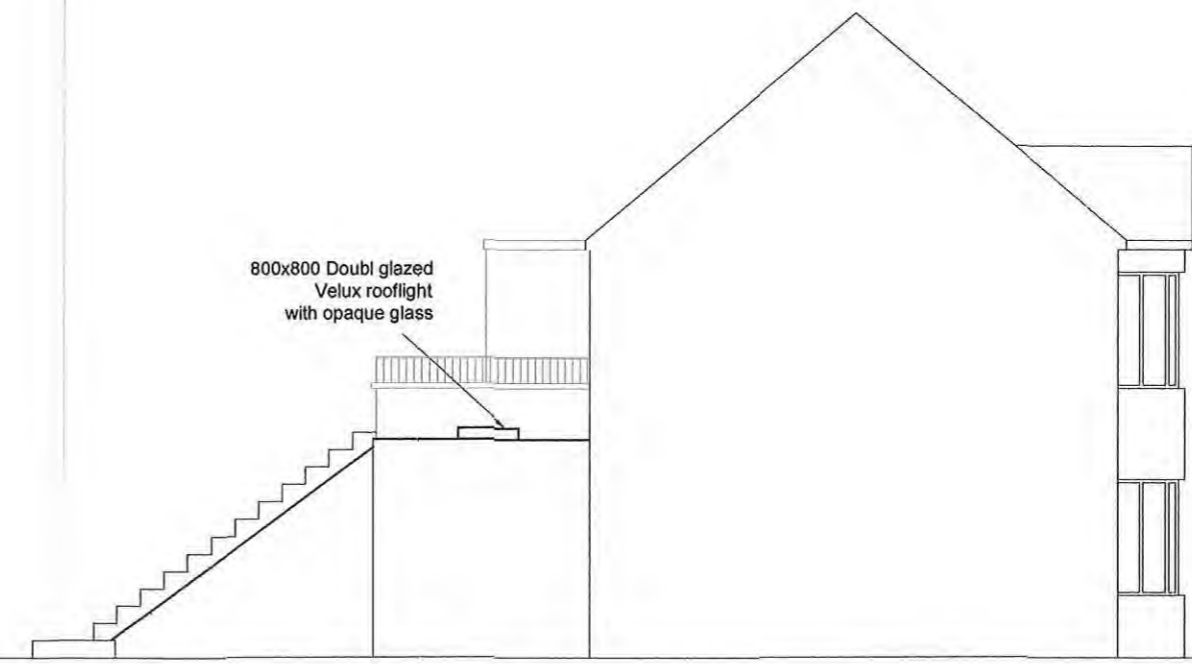
PROPOSED SECTIONAL ELEVATION X-X
