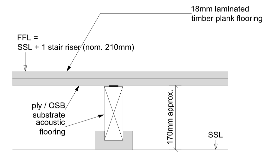
Typical Service/Acoustic Floor Detail 1:5
