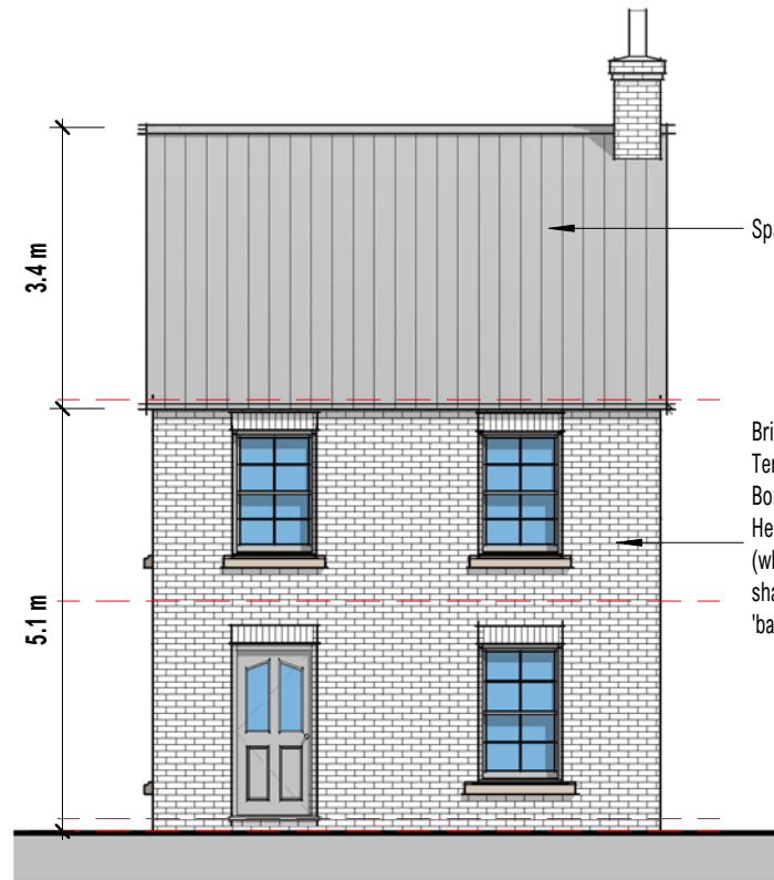
Elevation 01 - Front (north)
