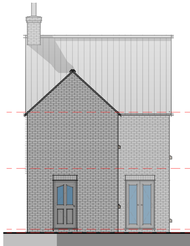
Elevation 03 - Rear (south)
