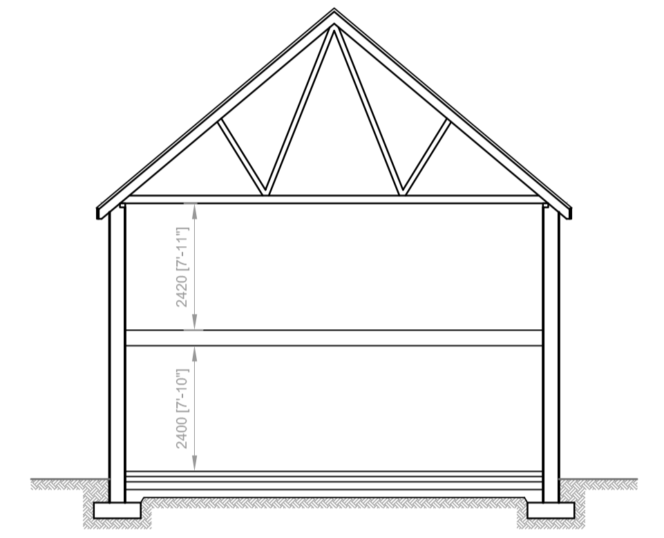
TYPICAL SECTION DETAIL
