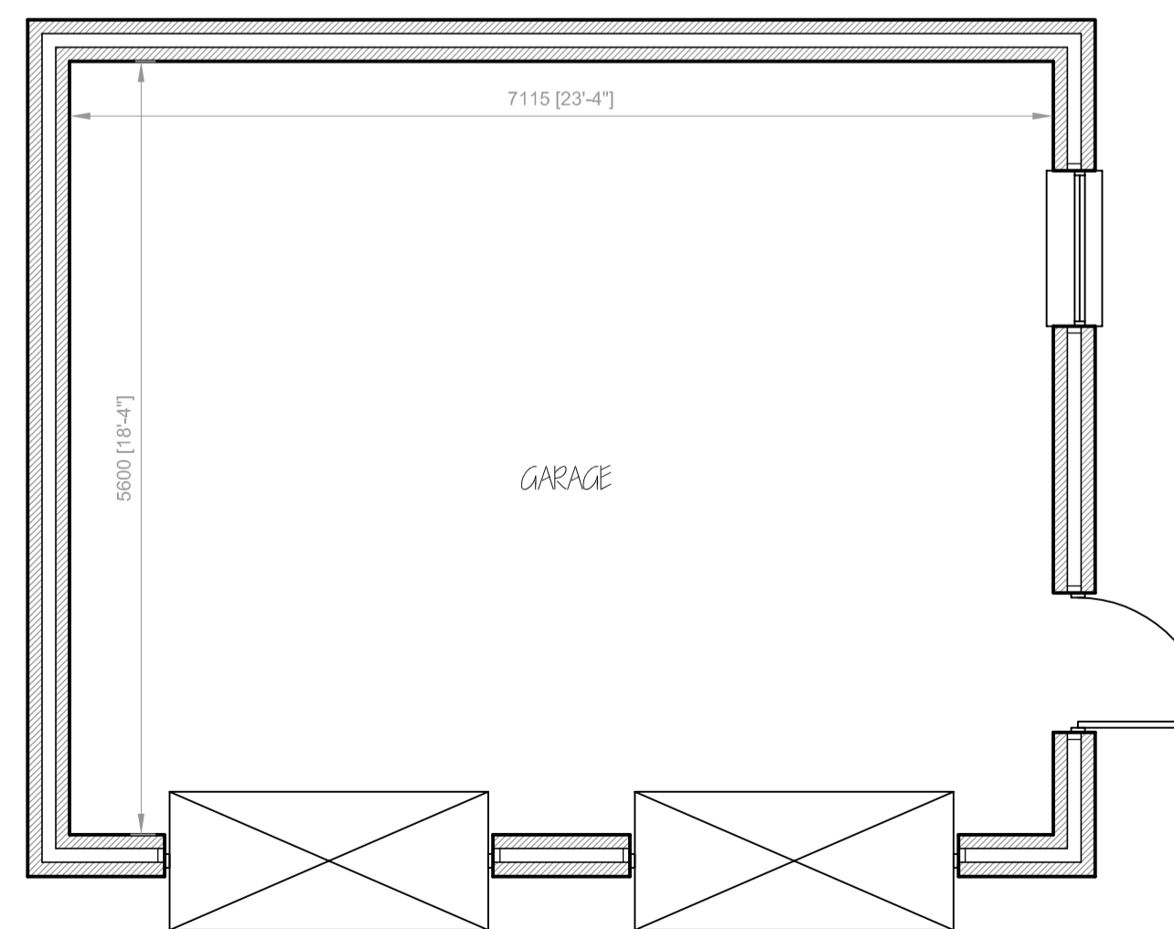
PROPOSED GARAGE FLOOR PLAN
