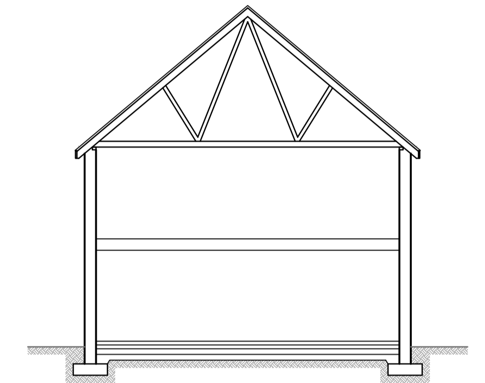
TYPICAL SECTION DETAIL
