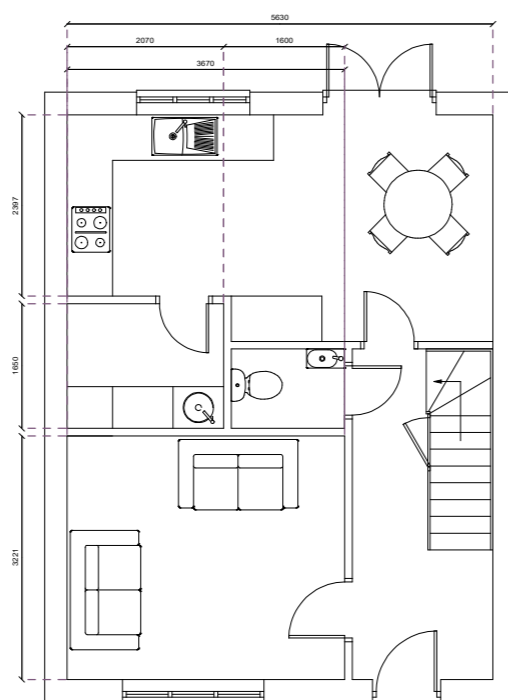
Ground Floor GIA - 42.04 m2 Total GIA - 84.08 m2
