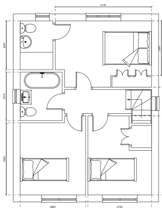
First Floor GIA - 42.04 m2
