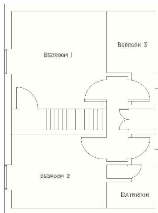
Proposed and Existing First Floor Plan
