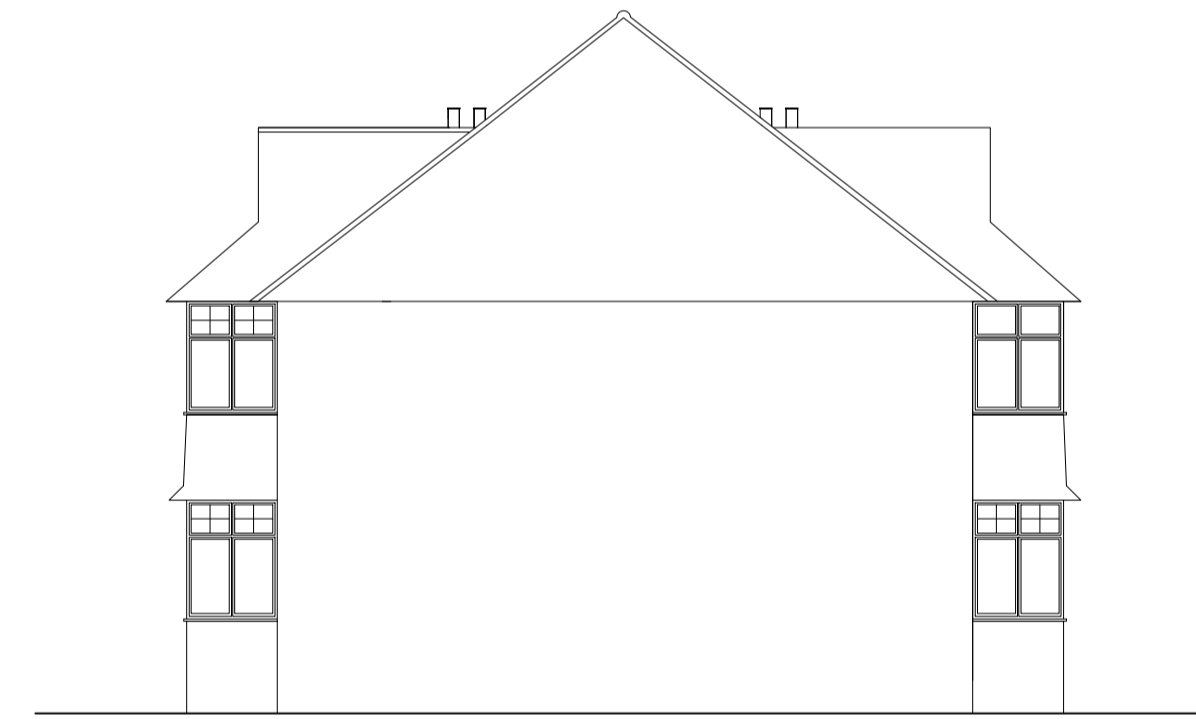
PRE Existing West Side Elevation
