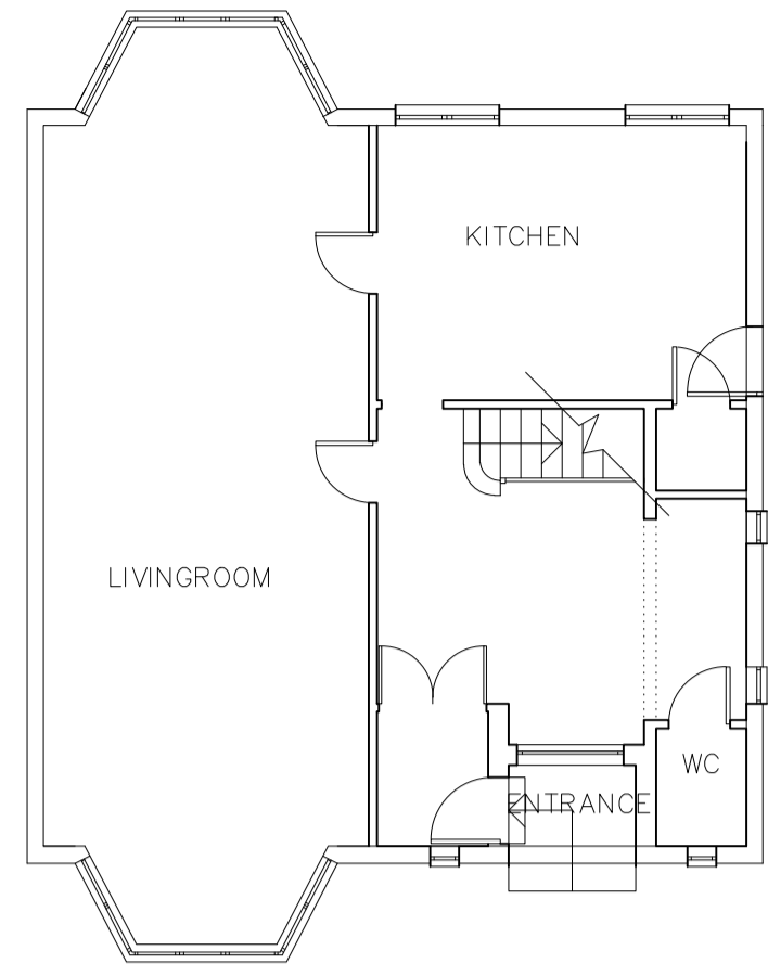
PRE EXISTING GROUND FLOOR PLAN
