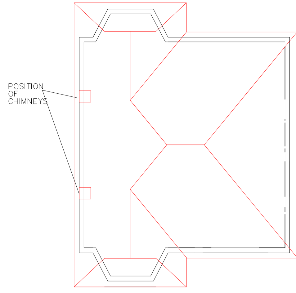
PRE EXISTING LOFT FLOOR PLAN
