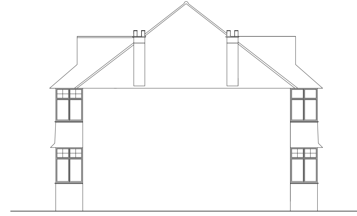
PRE Existing East Side Elevation
