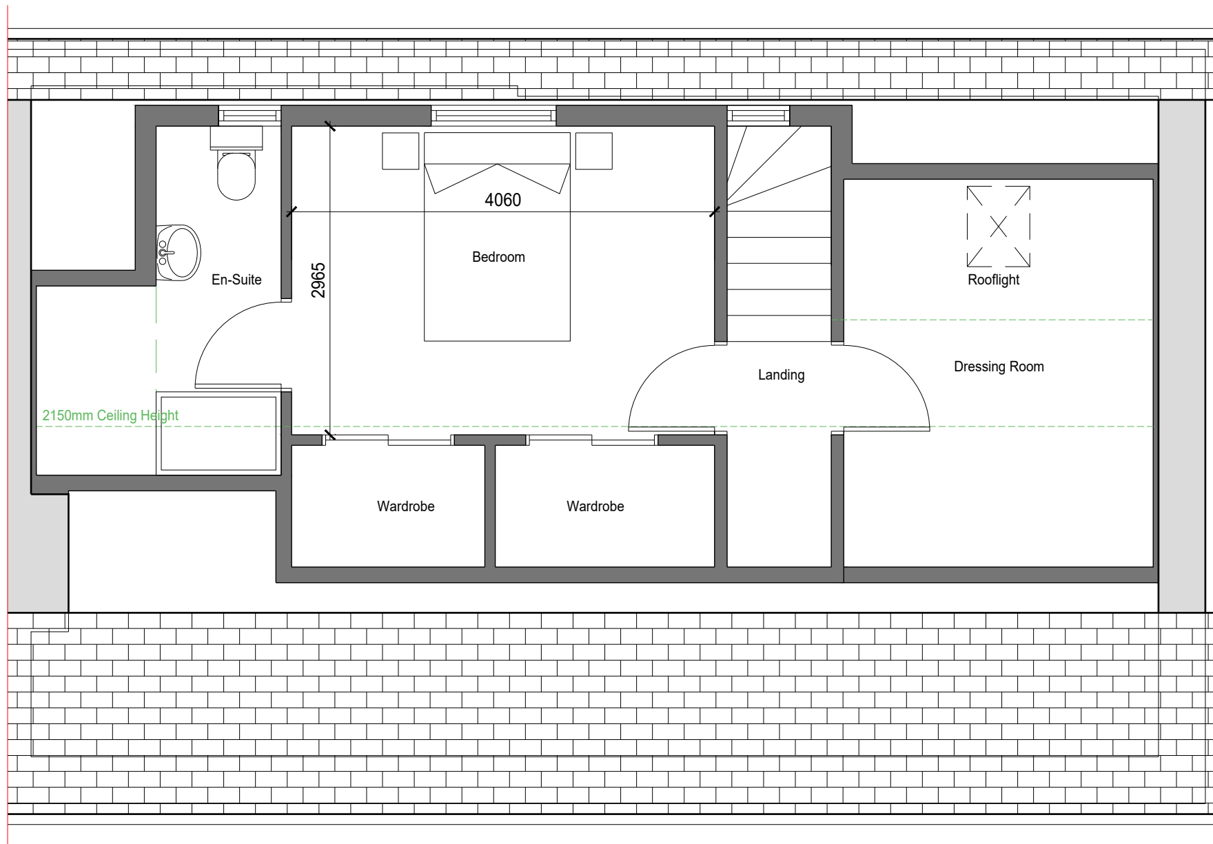
Proposed First Floor Layout Plan
