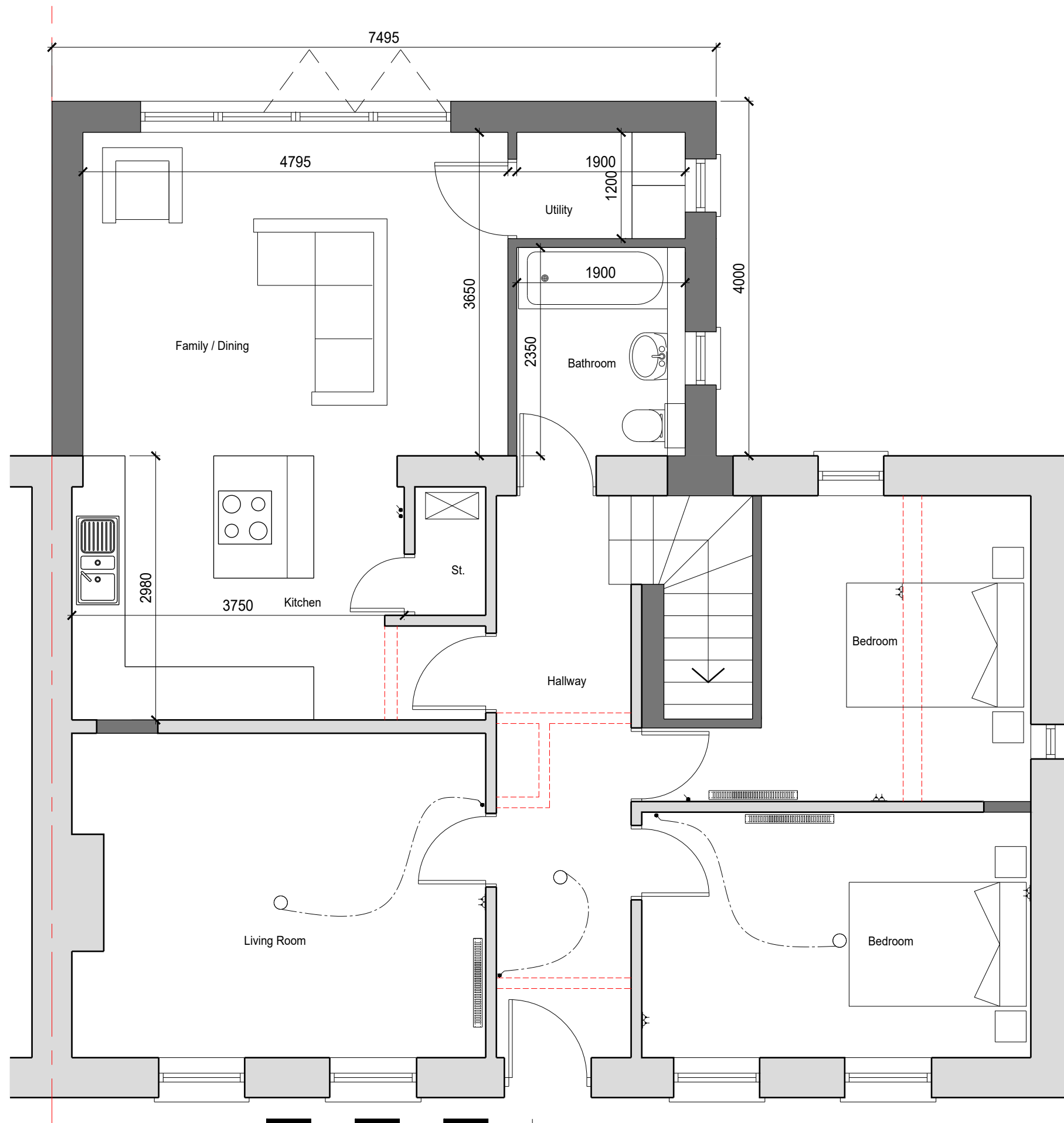
Proposed Ground Floor Layout Plan
