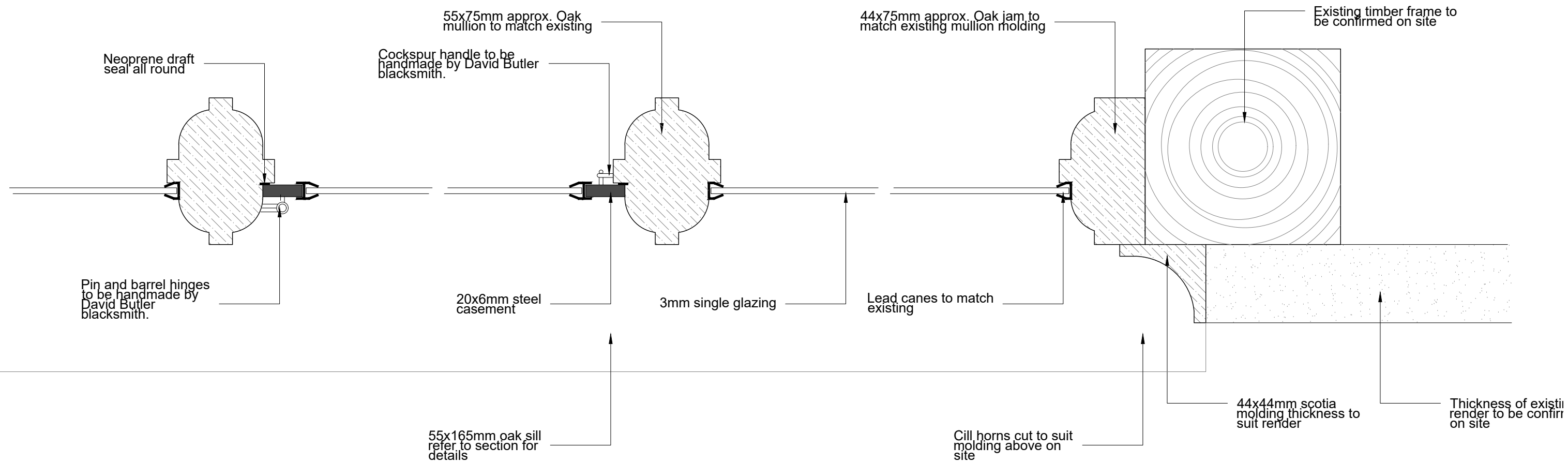
TYPICAL OAK MULLION PLAN ON 7-7 1:2
