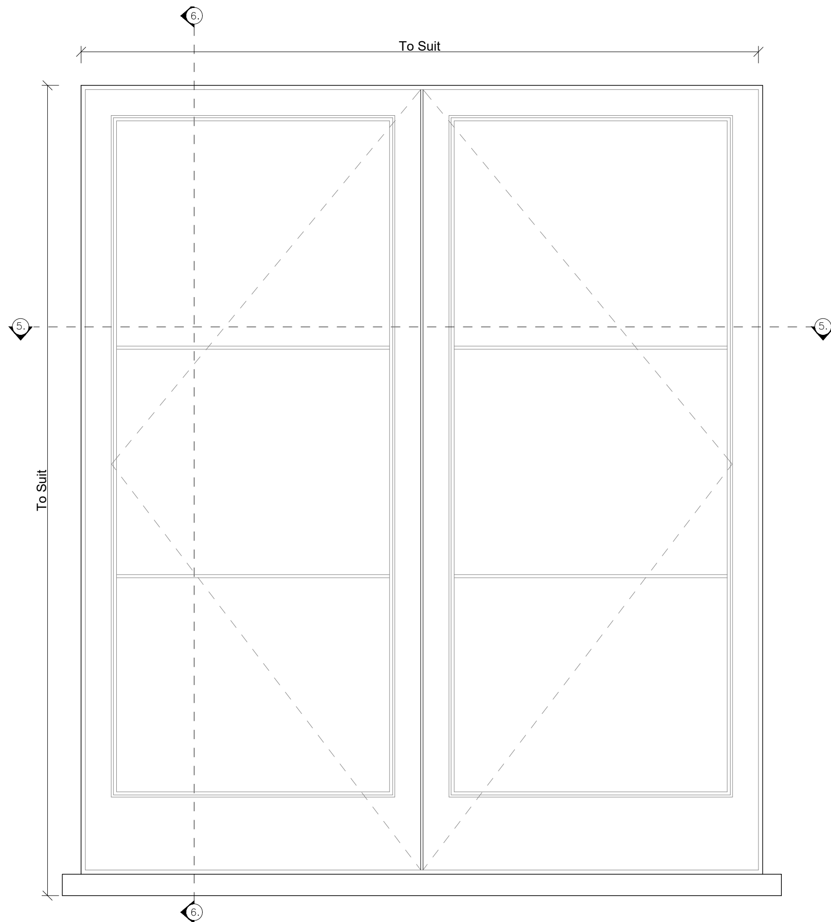
TYPICAL PATIO DOOR EXTERNAL ELEVATION 1:10
