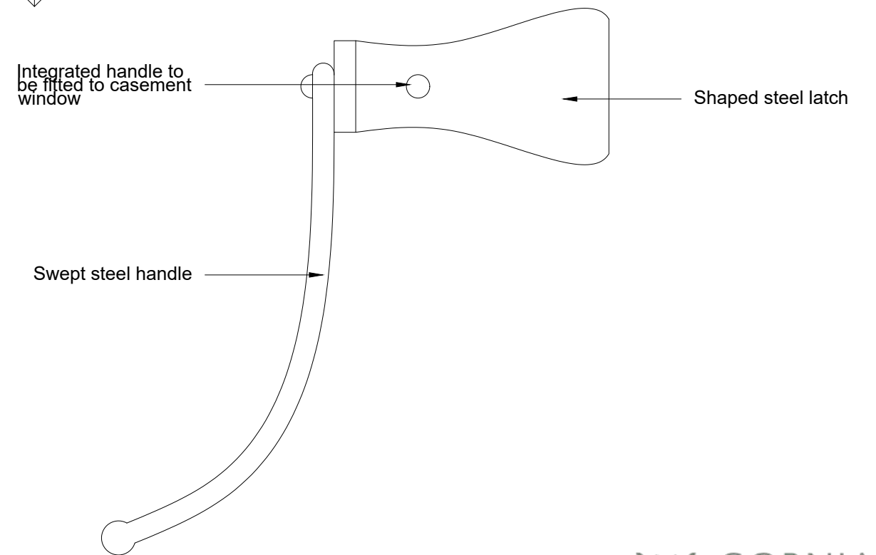
IRONMONGERY DETAILS 1:1
