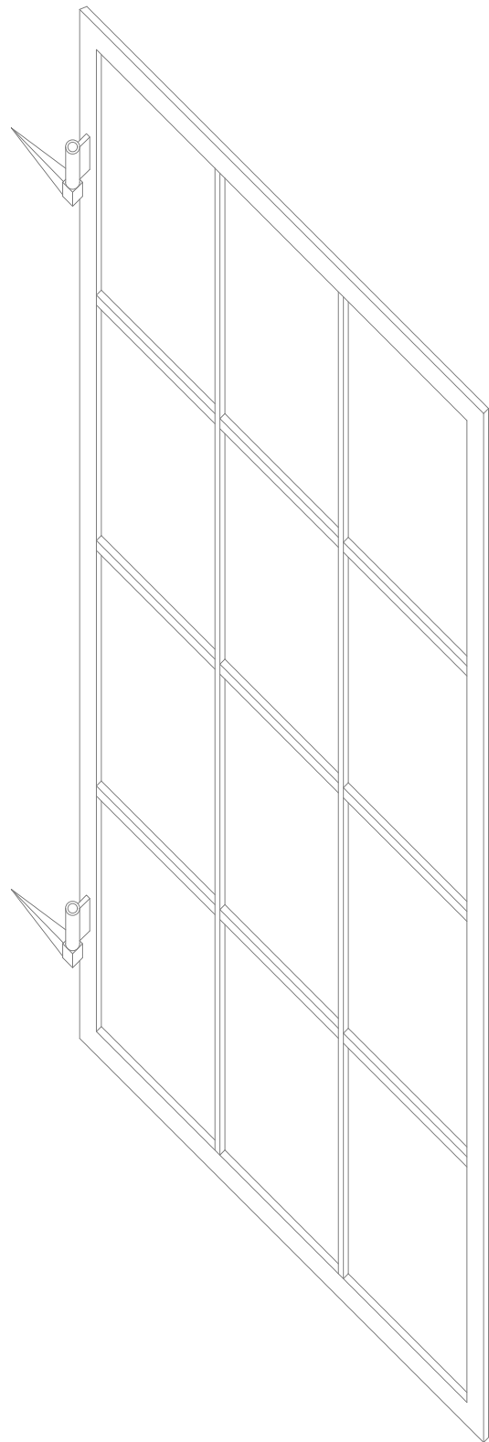
TYPICAL MULLION CASEMENT ISOMETRIC DRAWING NTS
