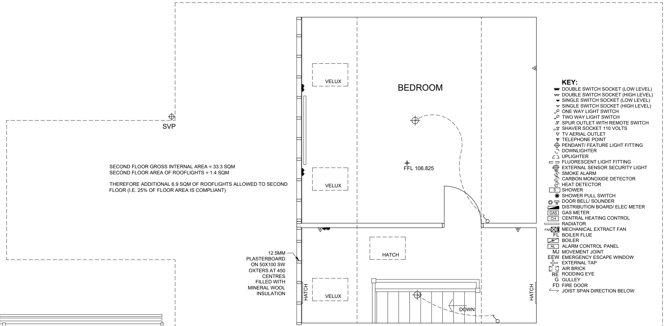
EXISTING SECOND FLOOR PLAN 1:50
