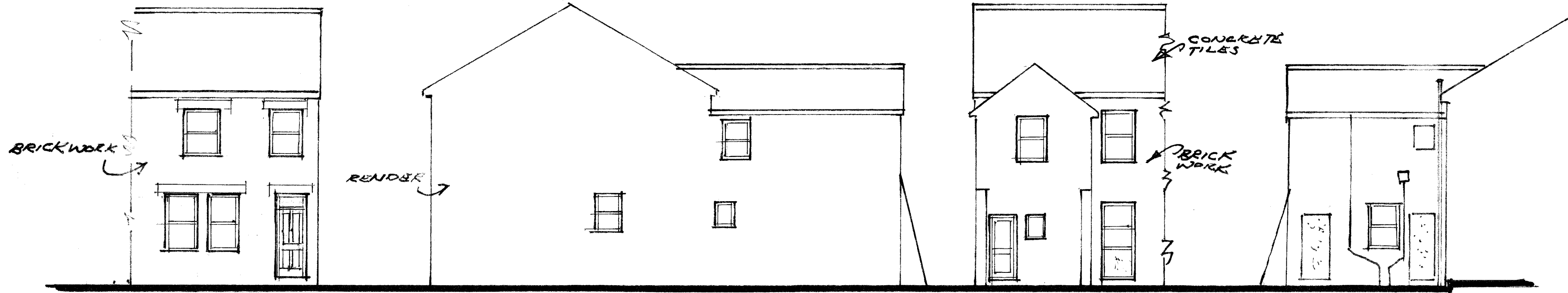
FRONT ELEVATION
