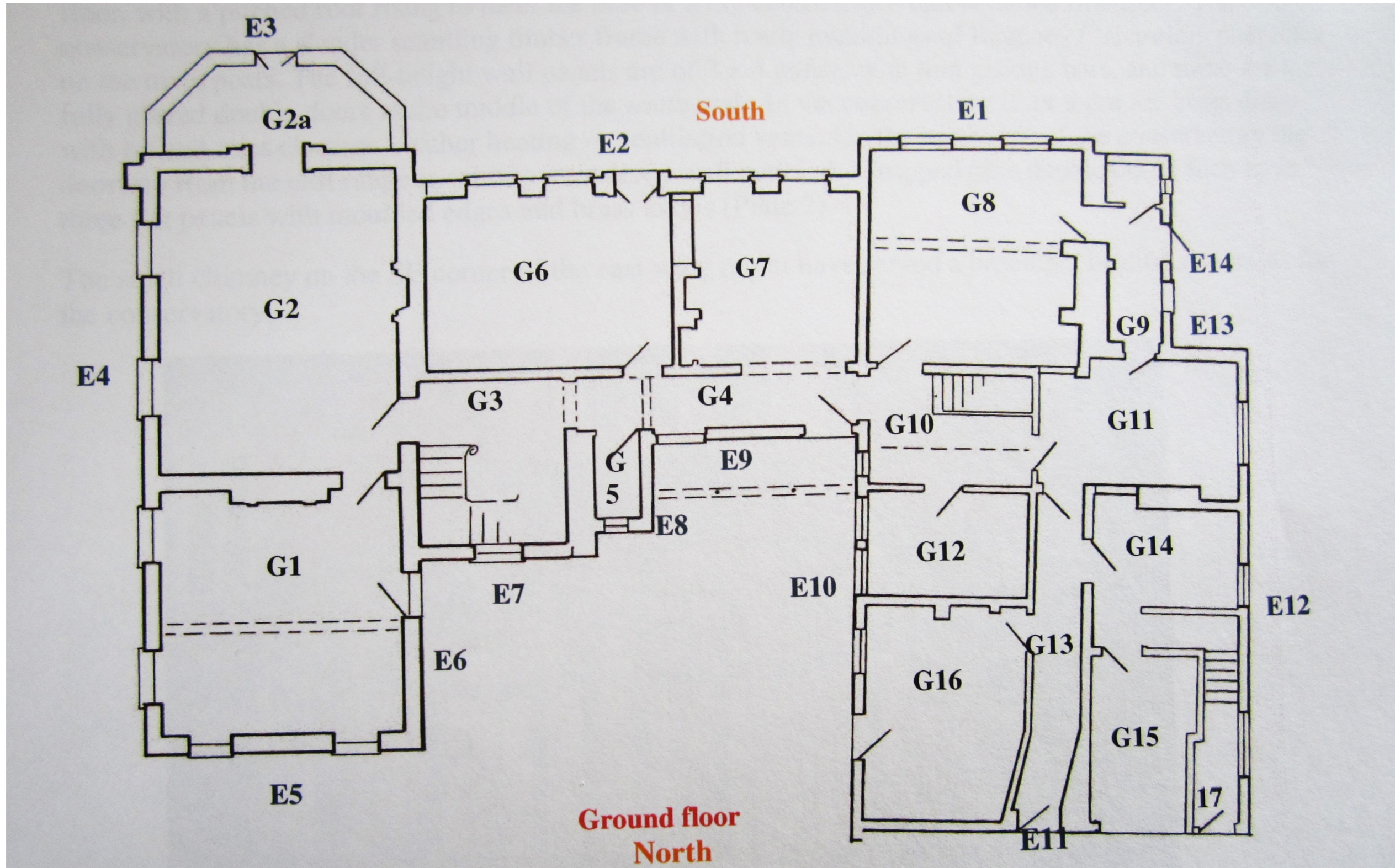
Drawing No. 1. Ground floor plan survey 1:100 @ A3, by Bob Meeson. Doorway proposed is between G7 and G8.
