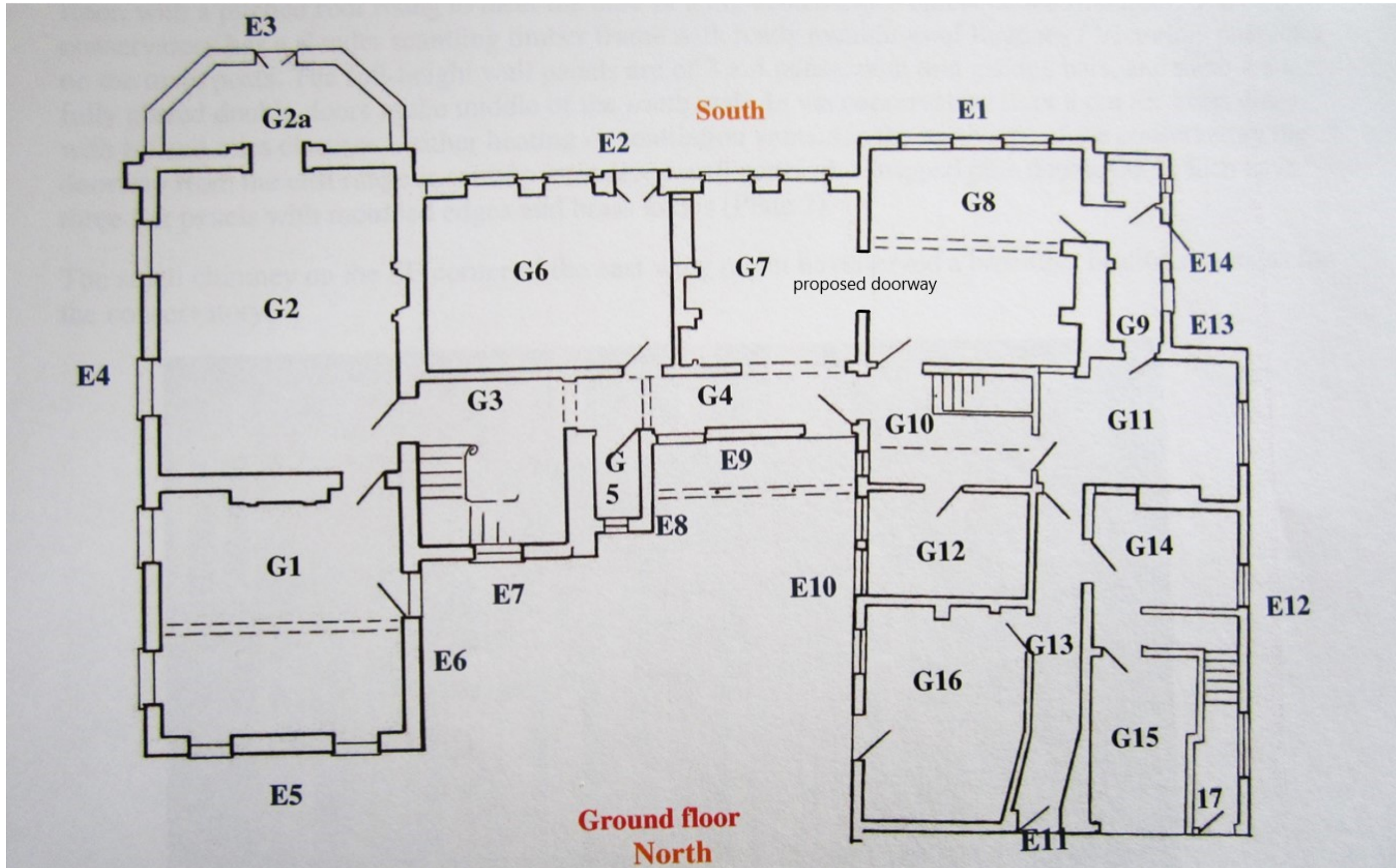
Drawing No. 2. Ground floor plan as proposed 1:100 @ A3 showing new doorway between G7 and G8.
