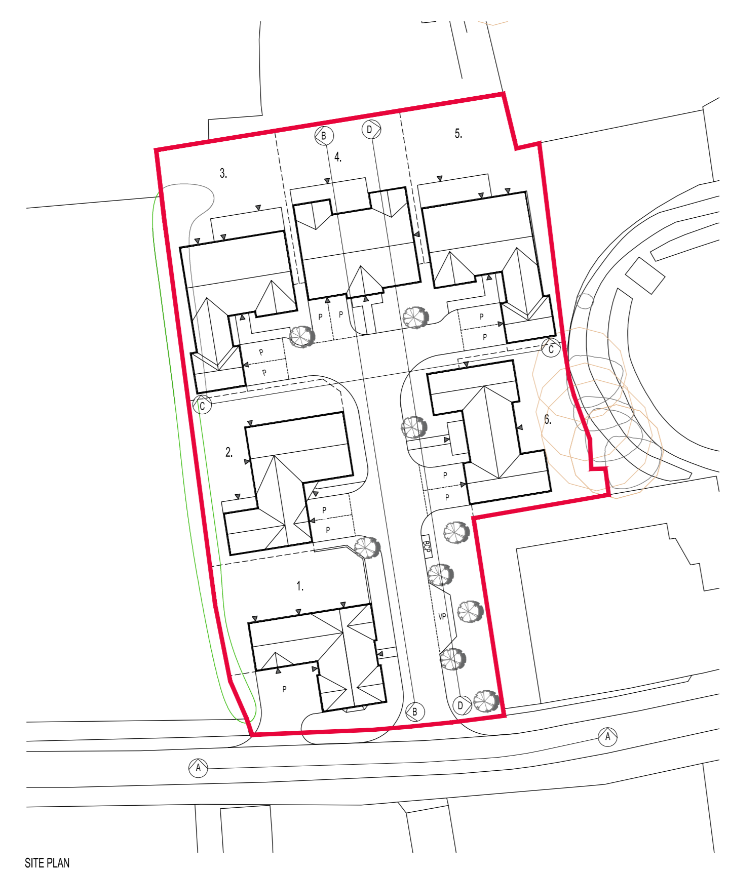
SITE PLAN
