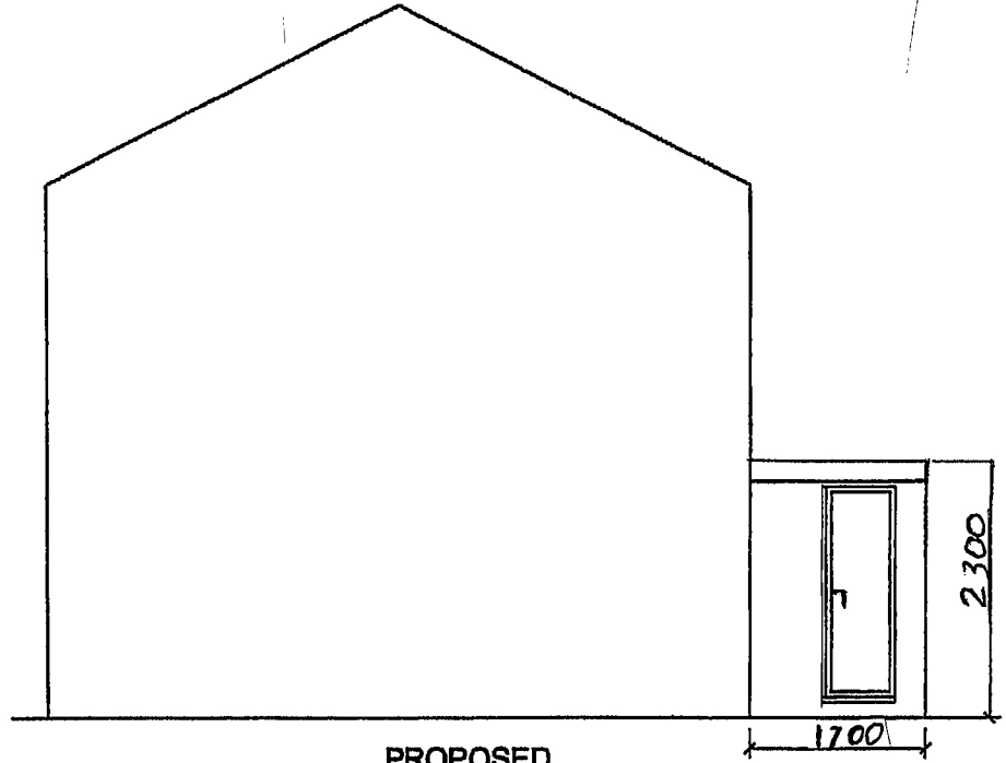
PROPOSED SIDE ELEVATION SCALE 1:50
