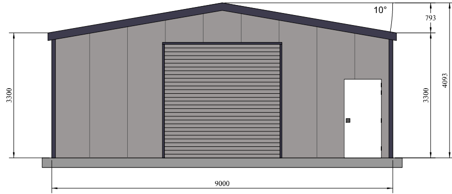
Front Elevation (External)
