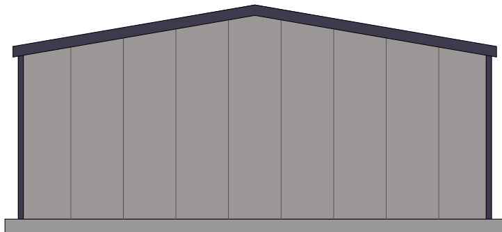
Back Elevation (Scale = 1:100)
