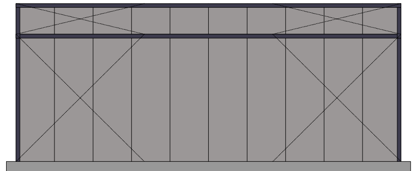
Right Elevation (Scale = 1:100)
