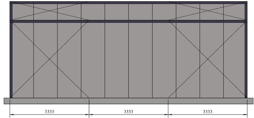
Left Elevation Internal (Scale = 1:100)
