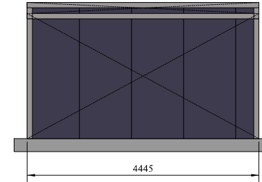
Left Elevation Internal (Scale = 1:100)
