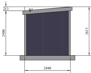
Front Elevation (External)
