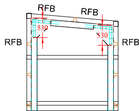
Back Elevation Frame (Scale = 1:100)
