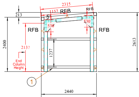
Front Elevation Frame (Scale = 1:100)
