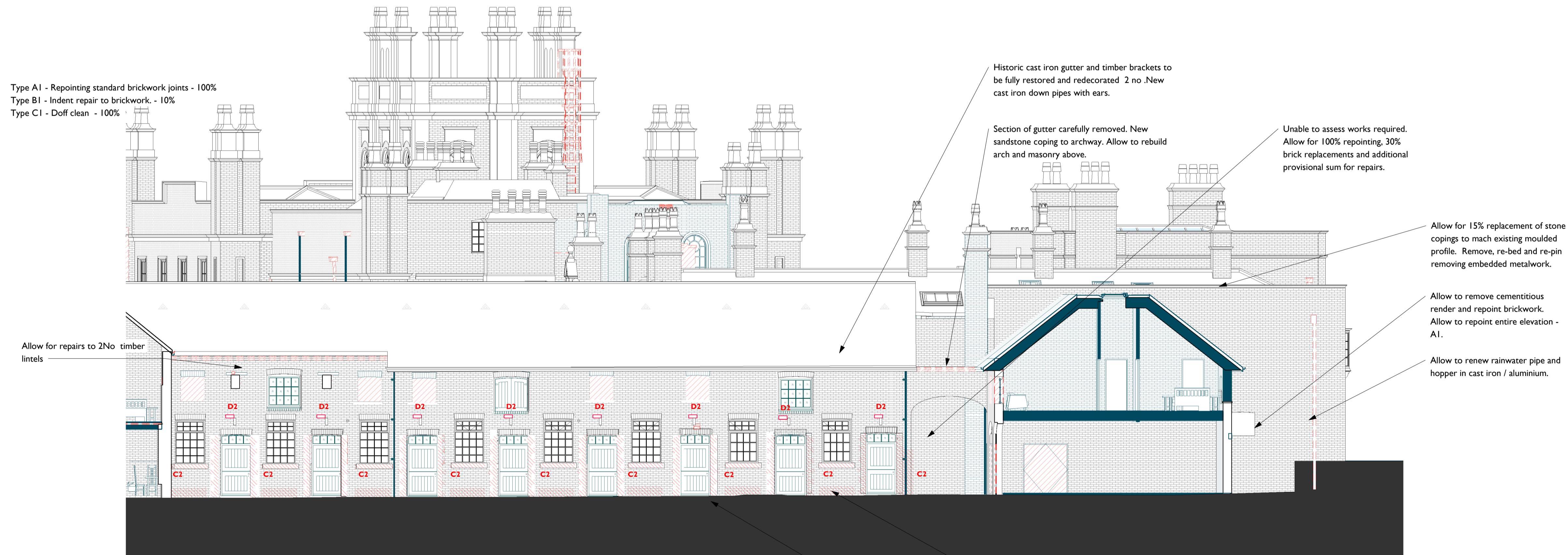
2 Stableyard Elevation 7 (SE7) Repairs w/Demo 1 : 100
