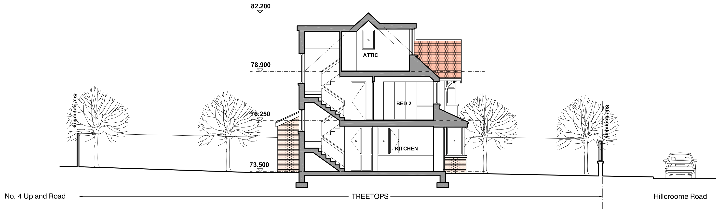
Proposed Section A-A Scale 1:100
