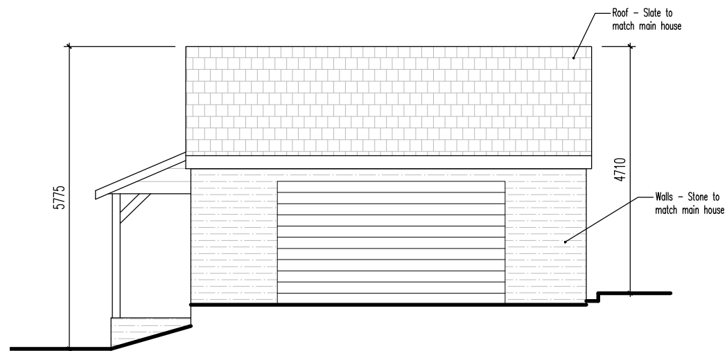
ELEVATION - FRONT
