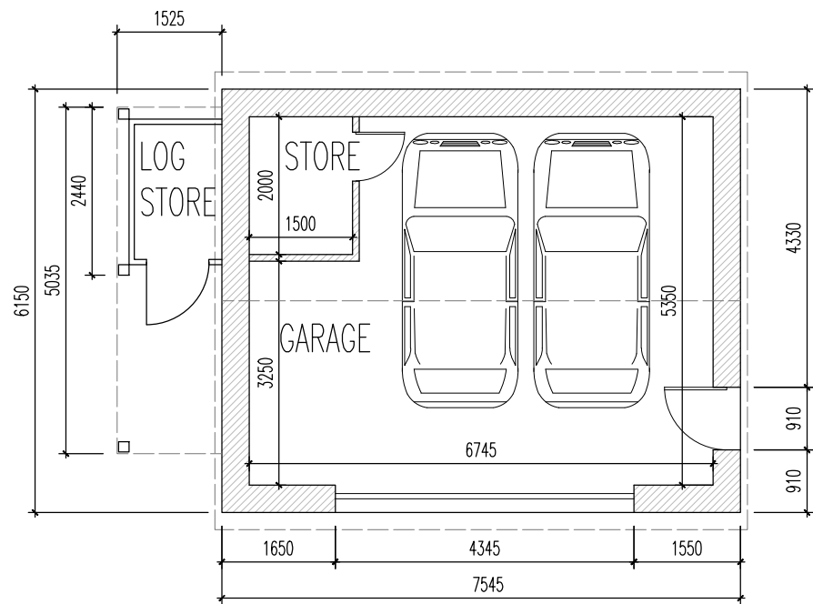
GARAGE PLAN LEVEL 0
