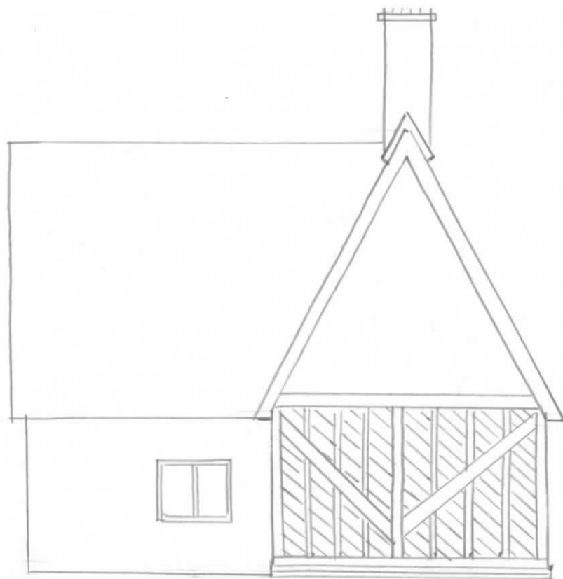
BACK ELEVATION
