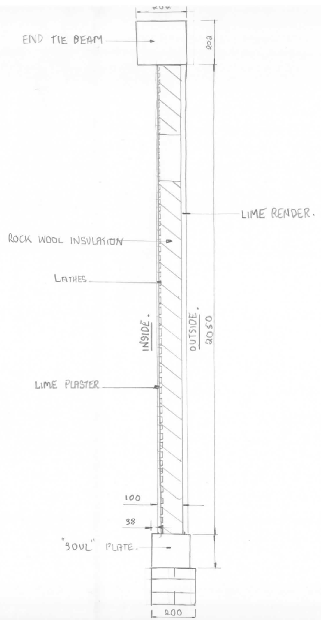
SECTION BB.
