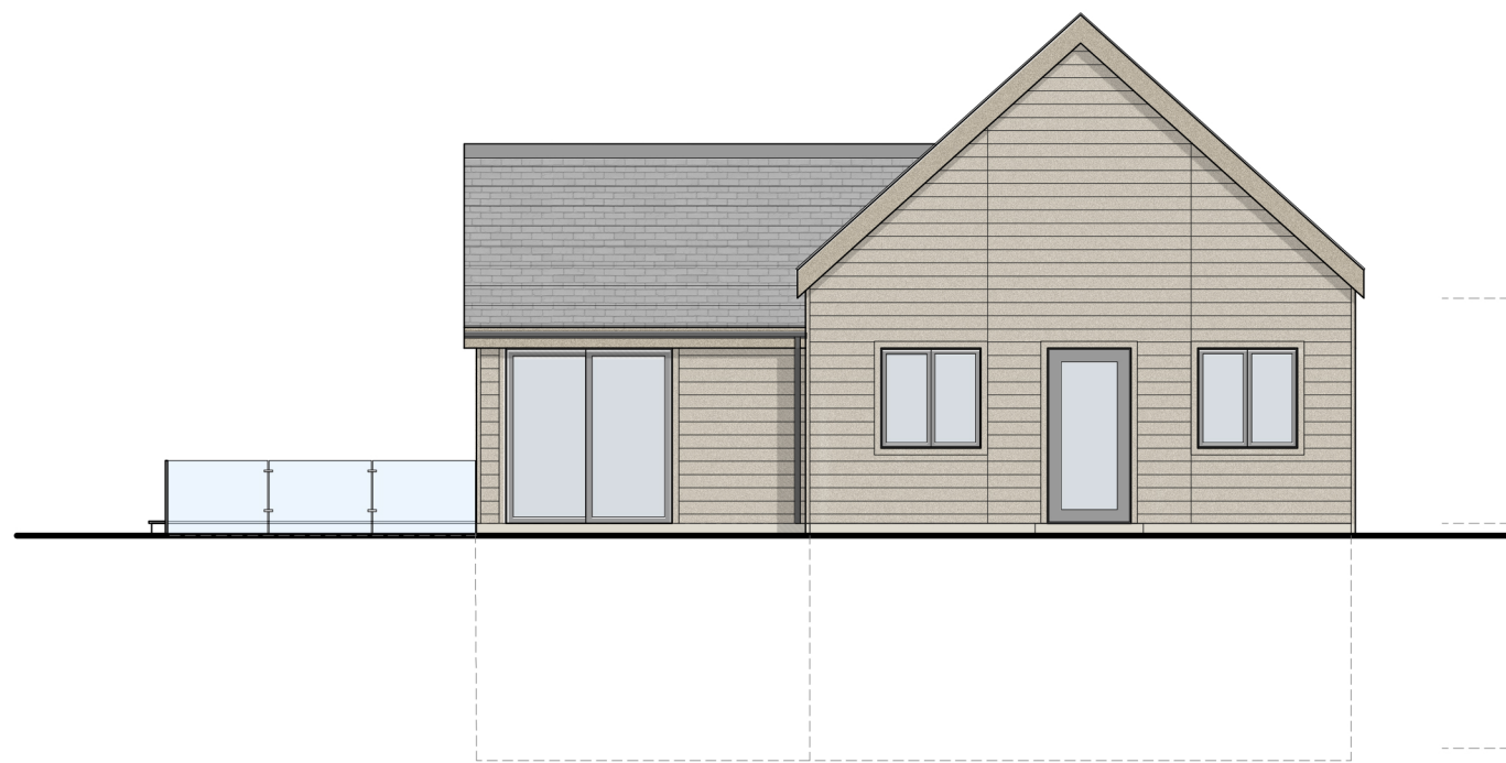
Rear Elevation [East]
