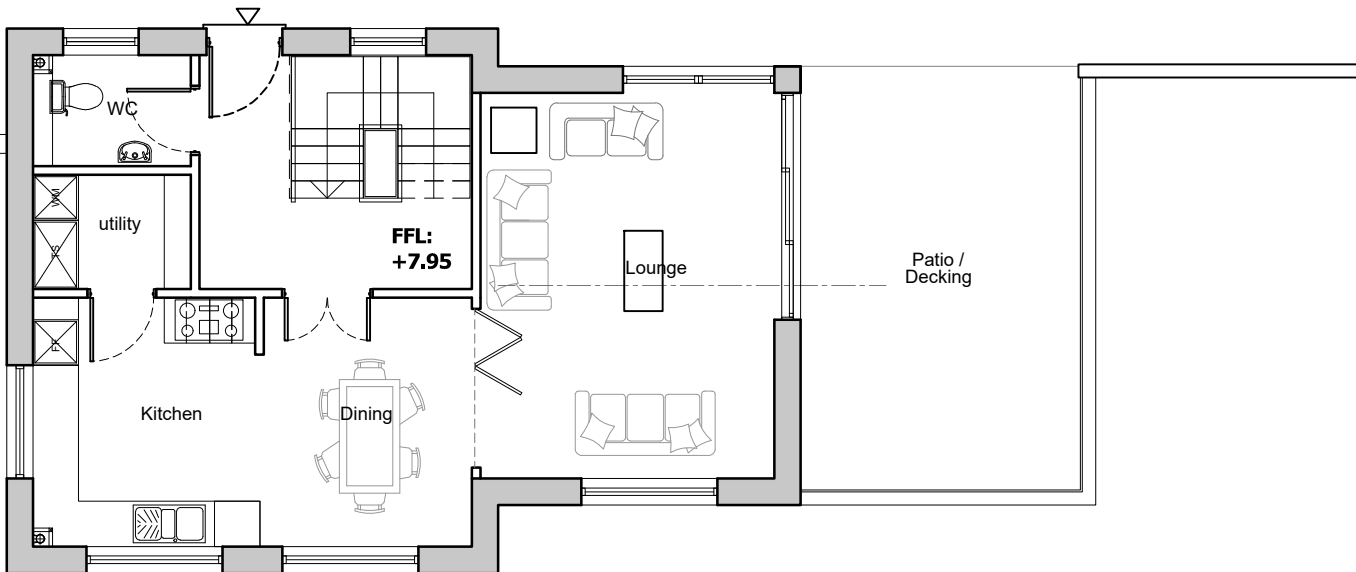
First Floor Plan [56.2m 2 ]
