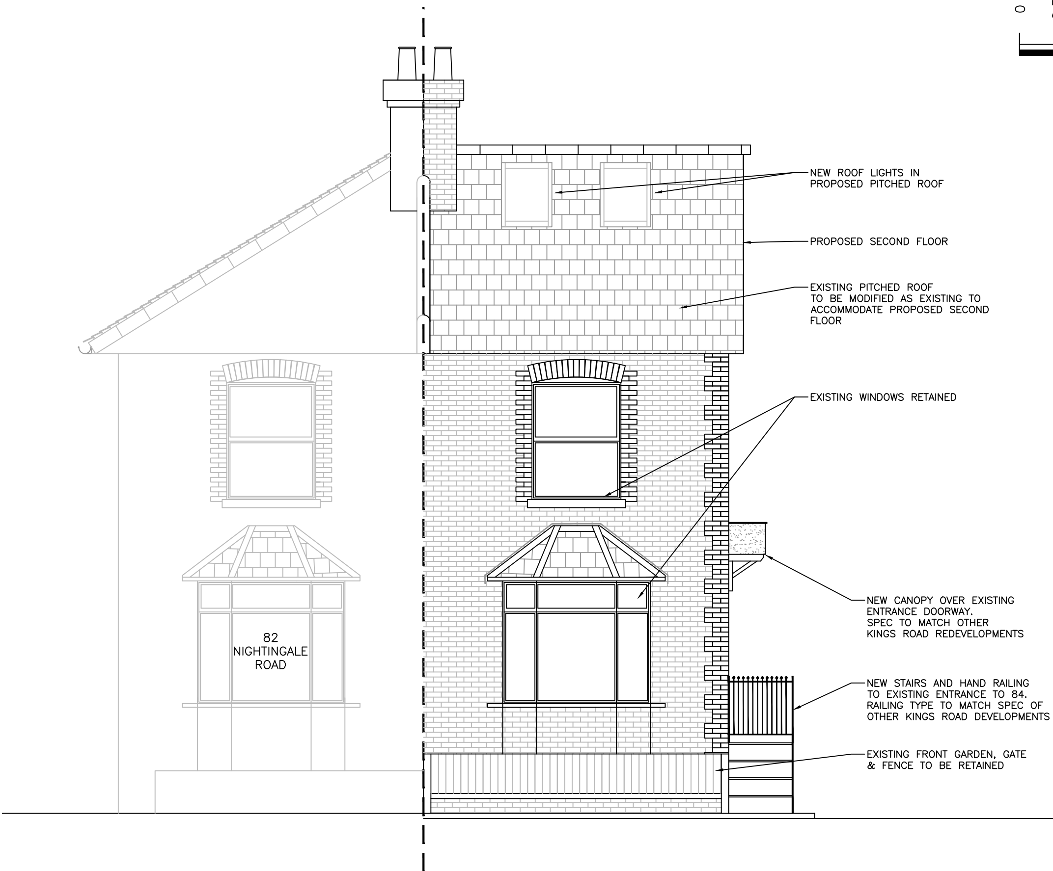
PROPOSED NORTH ELEVATION - 1:50 @ A3
