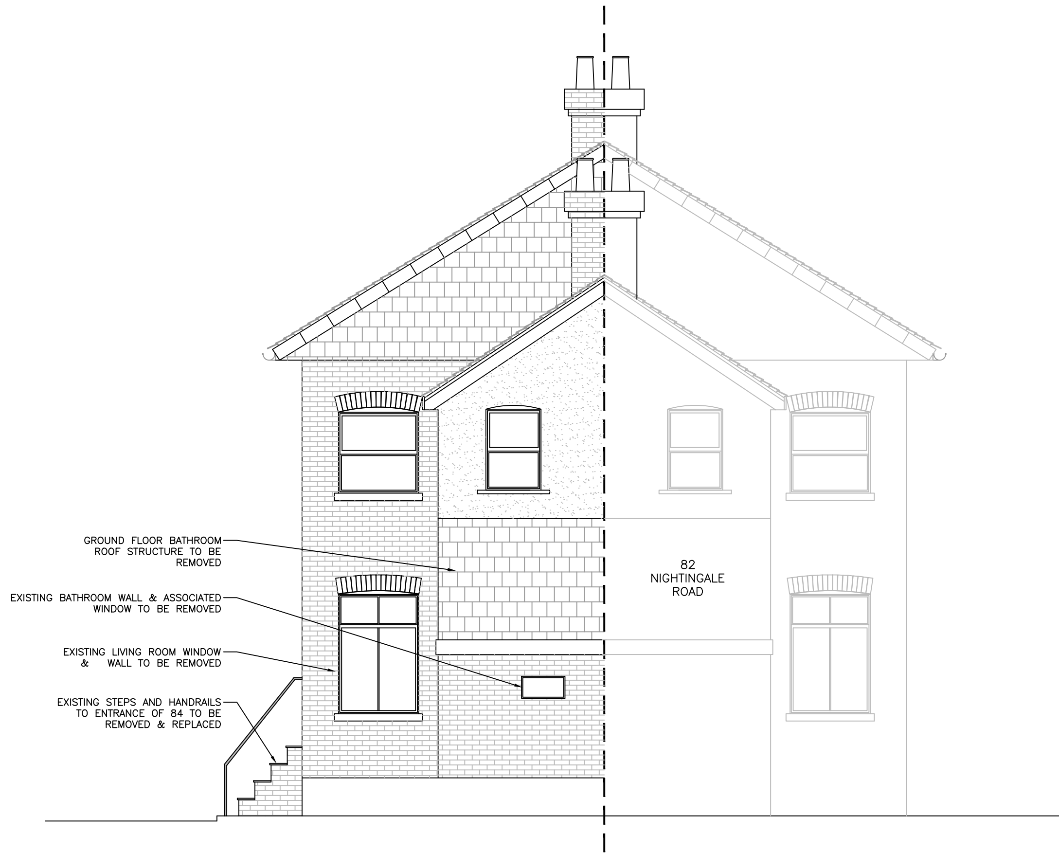
EXISTING SOUTH ELEVATION - 1:50 @ A3
