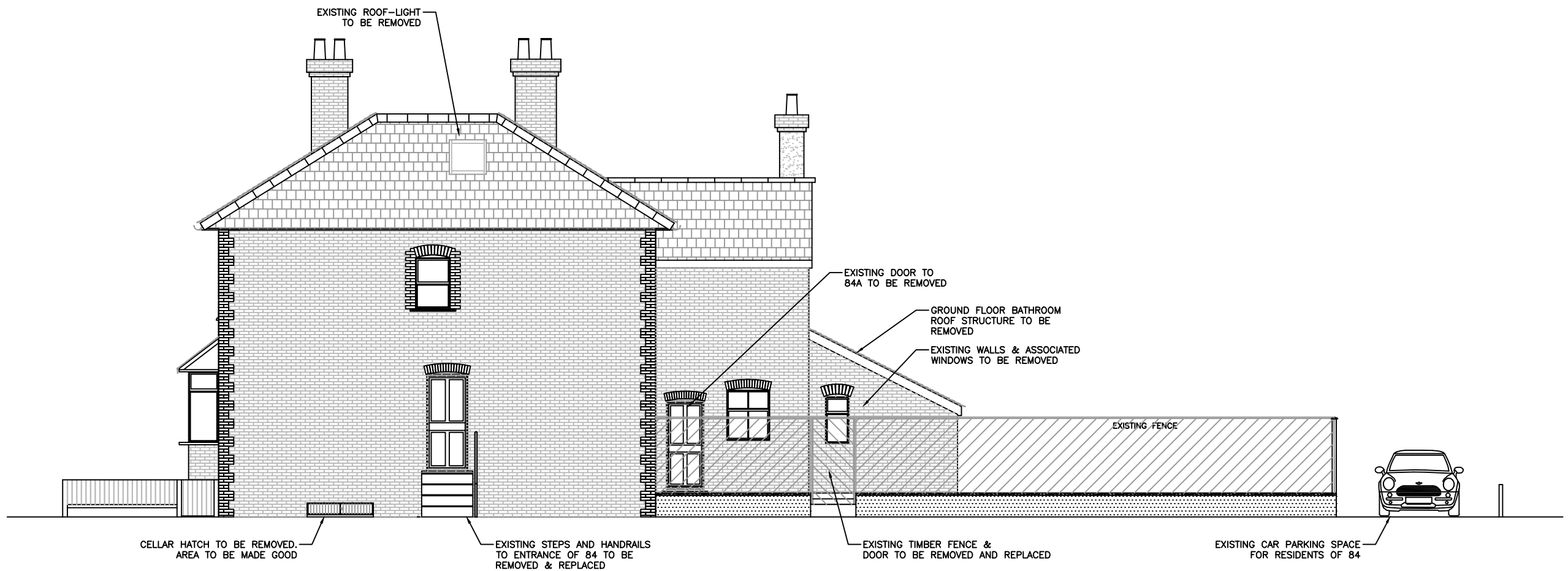
EXISTING WEST ELEVATION - 1:100 © A3
