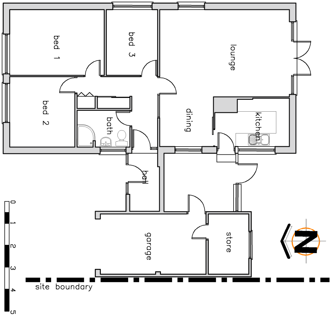
floor layout scale 1:100
