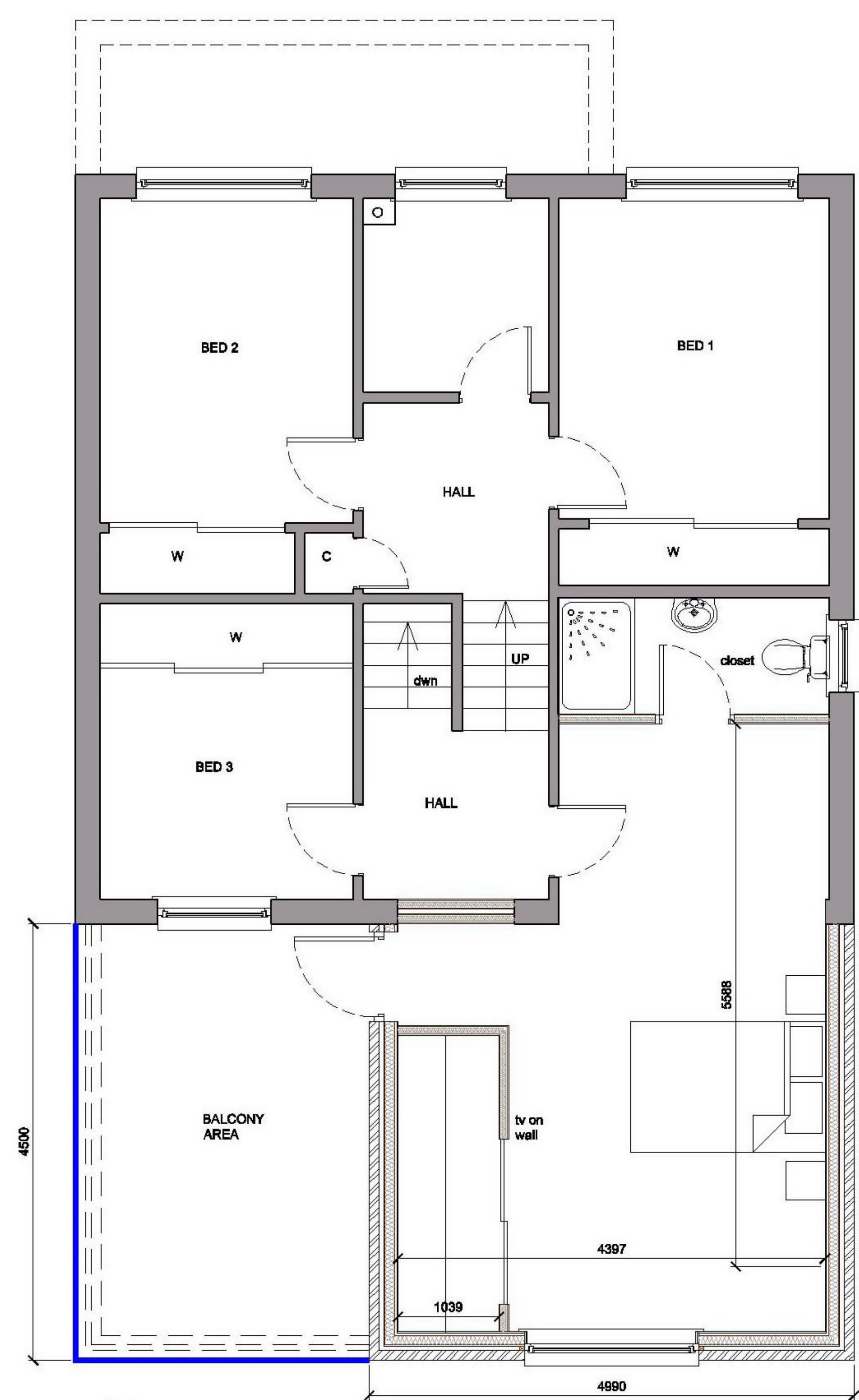
1:50 LOWER/UPPER FIRST FLOOR WALL LAYOUT AS PROPOSED
