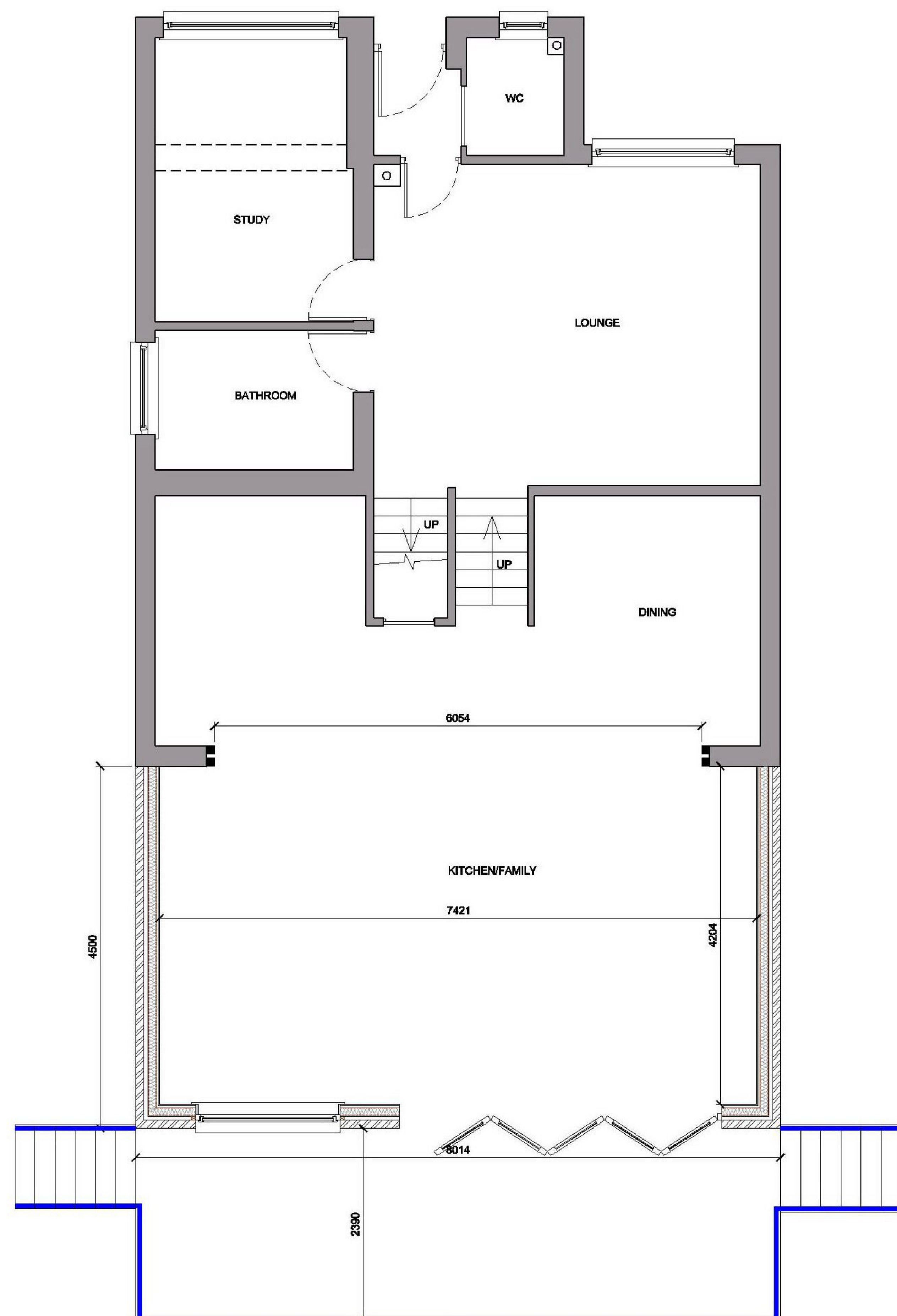
1:50 LOWER/UPPER GROUND FLOOR WALL LAYOUT AS PROPOSED
